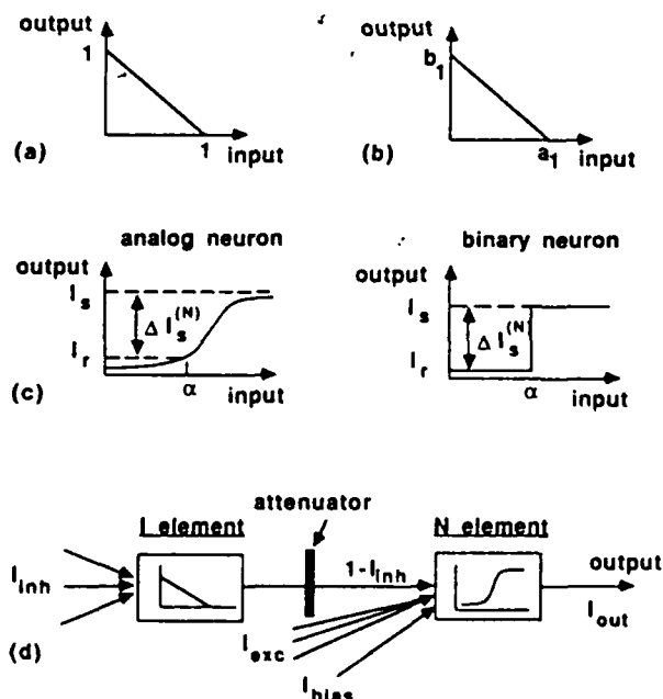
Fig. 1. The ION. (a) The inhibitory element; (b) the unnormalized inhibitory element; (c) the nonlinear element; (d) the structure.
