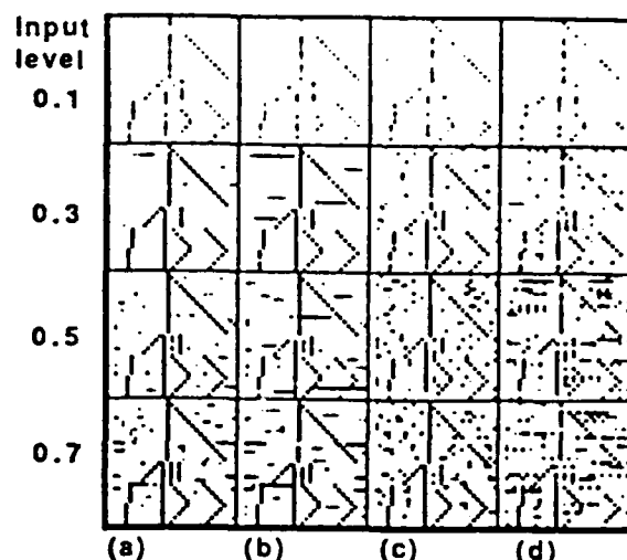
Fig. 9 Simulation result of spatially and temporally correlated noise. sc is the spatial correlation range. Three noise sources are simulated simultaneously with p = \pm 10\% and correlation period T .
