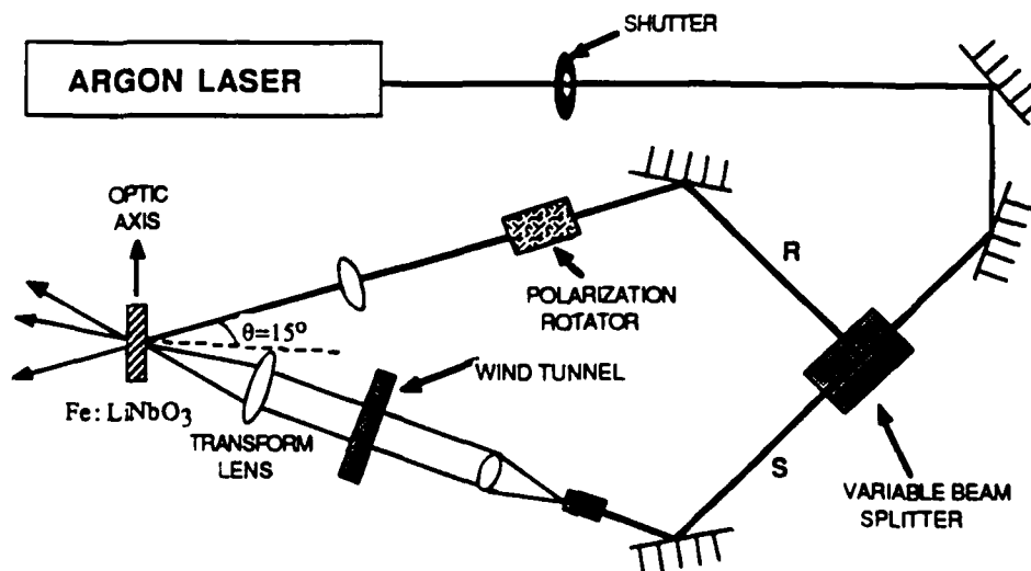
Figure 1 Experimental system.
