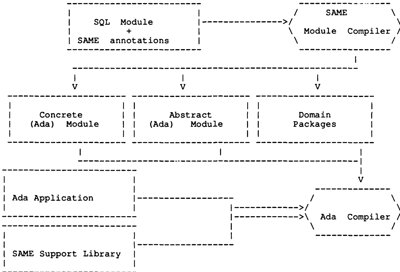
Figure 3: Possible SAME Tool Approach
