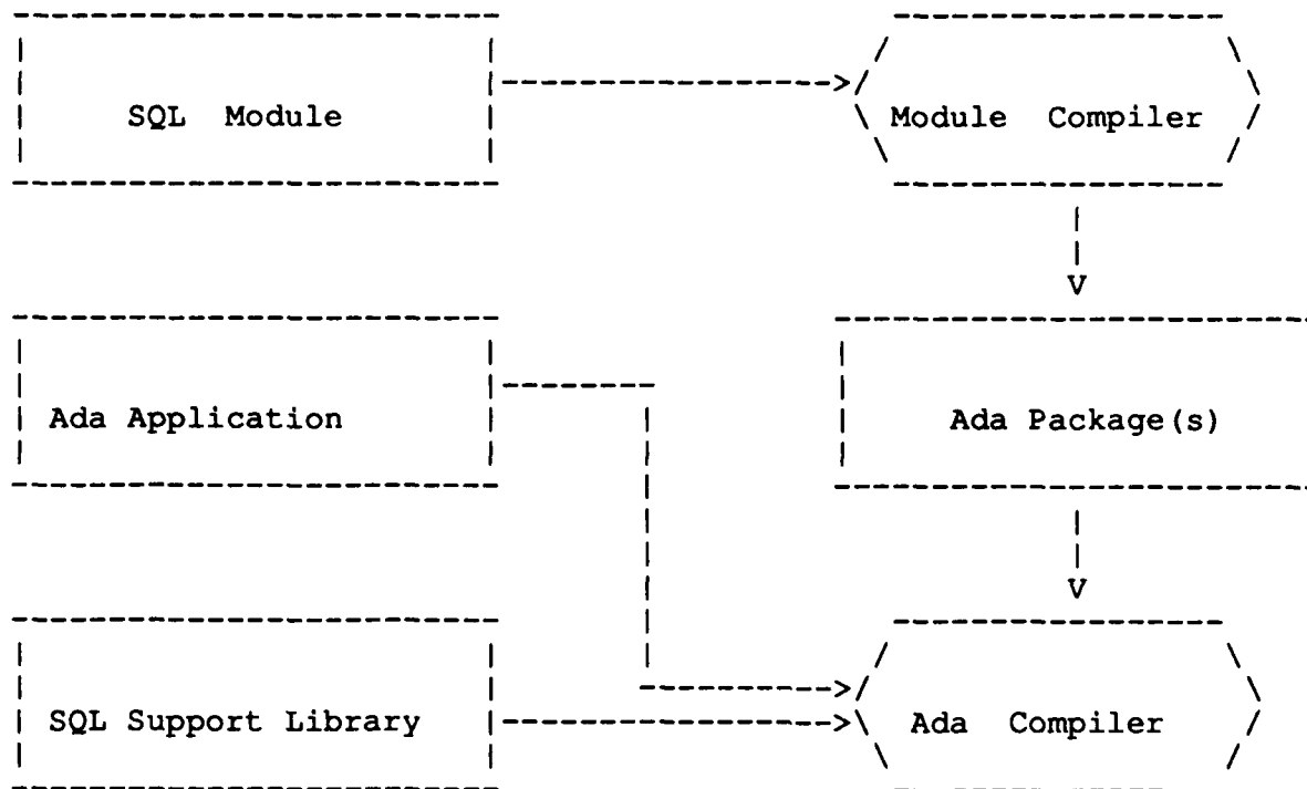
Figure 2: SQL Module Approach
