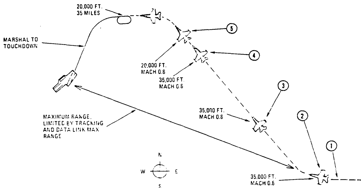
FIGURE 5-1 FLIGHT PATH, ENTRY TO HOLDING
