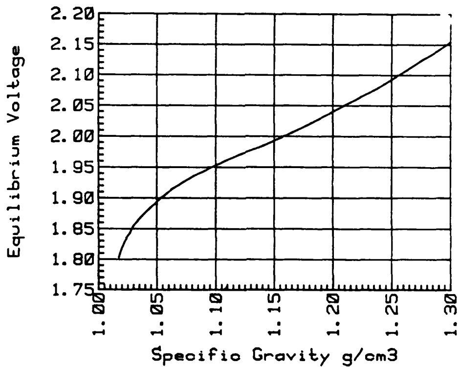
Figure 4. Electrolyte Density as a Function of Equilibrium Voltage
