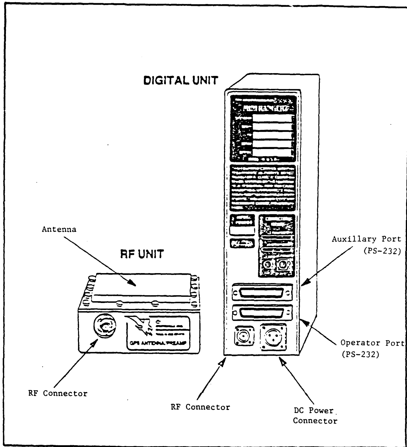
FIGURE A-1. EAGLE GPS RECEIVER
