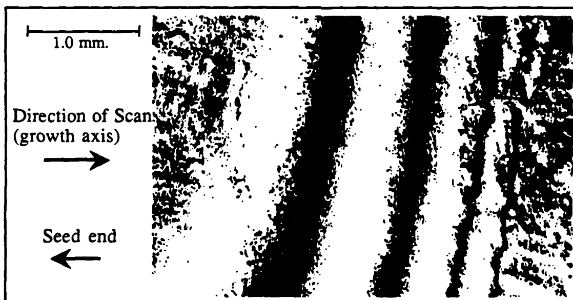
Figure 4.3 Fringe pattern in the image plane of the Mach-Zehnder interferometer for the index gradient region of crystal mh721.
