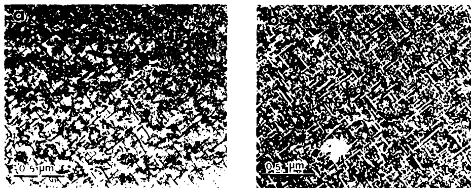
Figure 6. TEM's of the 2090 alloy solution heat treated showing a complex precipitate structure that includes \theta' , T_1 , \delta' , and \text{Al}_3\text{Zr} ( R' ). (a) Bright field, (b) dark field.
