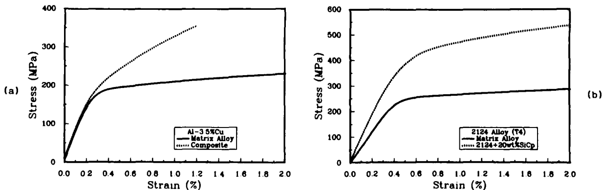
Fig. 16. The shape of stress-strain plots for (a) an Al-3.5%Cu alloy with and without 20% by vol. of \delta-Al_2O_3 short fibres and (b) 2124 alloy with and without 20 wt.% SiC ( \approx 17 vol.%) particles.
