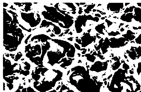
Fig. 19. Fracture surface of (a) 3.2 \mu m and (b) 20 \mu m average particle size SiC/Al composite (after Ref. 43).
