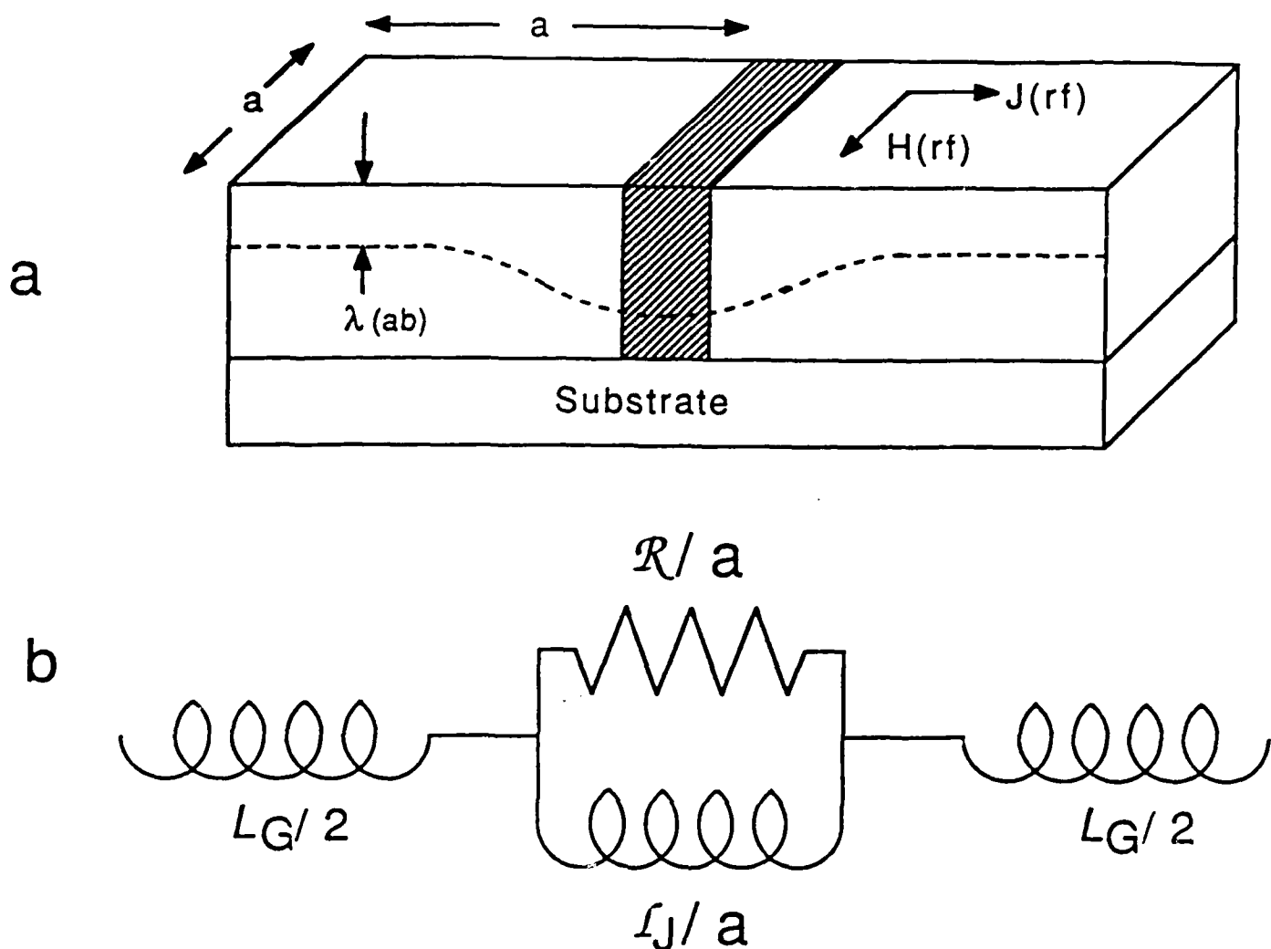
Figure 1a. Two grains of dimension a are coupled by a weakly superconducting region (shaded) in this idealization of a grain boundary junction of a thin film. The currents are confined to a penetration depth as in a typical surface impedance measurement. The dashed curve is a profile of the penetration depth of the currents into the grain and grain boundary. b. A circuit model of figure 1a consists of purely inductive grains in series with a grain boundary of parallel inductive and resistive channels.
