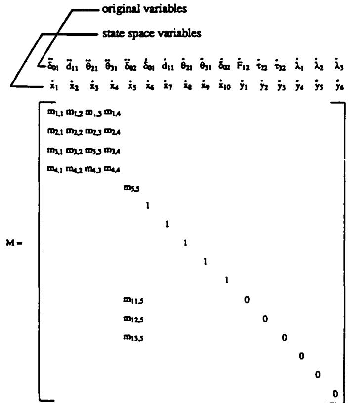
Fig. 7 Dynamic Equations in State Space Form for Two Rigidly Connected, Planar Manipulators on Independent, Vertically Compliant Bases
