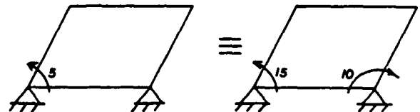
Fig. 4 An Example of Actuator Conflict for a Non-Compliant, Four Bar Linkage
