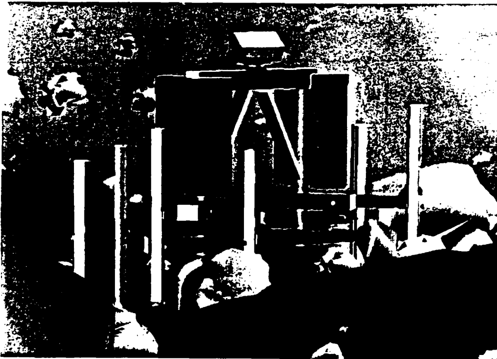
Figure 5: Simulated Ambler on synthetic terrain
