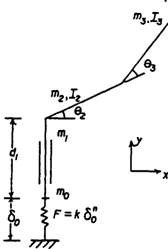
Fig. 1 Planar Manipulator on a Vertically Compliant Base
