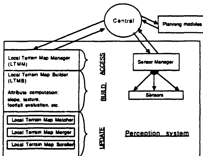
Figure 2: Architecture of the perception system
