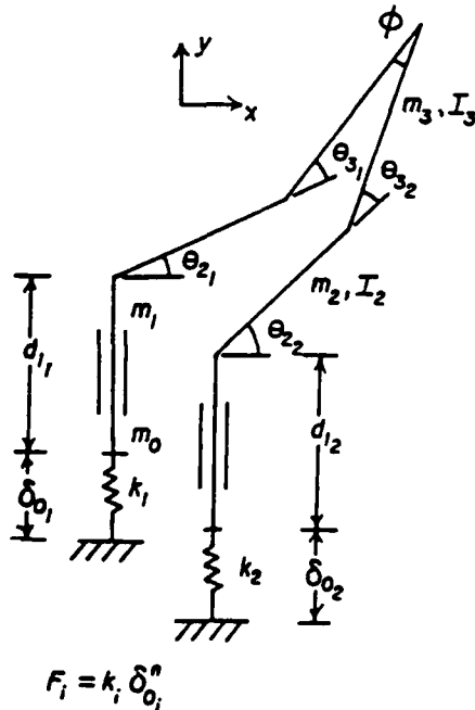
Fig. 5 Two Rigidly Connected, Planar Manipulators on Independent, Vertically Compliant Bases
