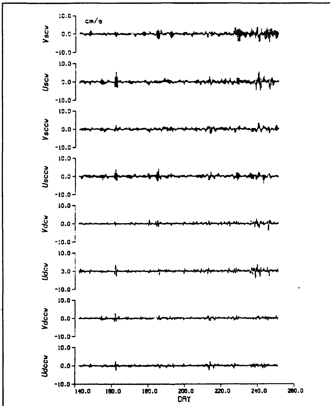
Figure C1 Buoy 4980.
