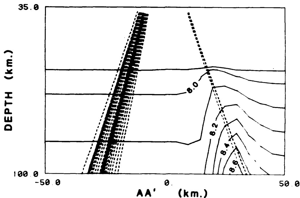
Figure 1b Iso-P velocity contours greater than 7.9 km./sec for the Taylor (1983) model along the AA' cross section shown in Figure 1. Three-dimensionally traced rays (dashed) are projected onto the cross section if their end points lie within 20 km. of the plane of the cross section.
