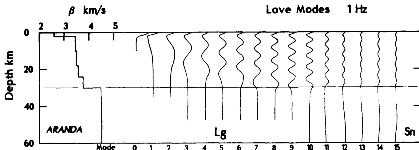
Figure 1: ARANDA reference model and Love mode eigenfunctions with phase velocity less than 4.54 km/s at frequency 1 Hz.
