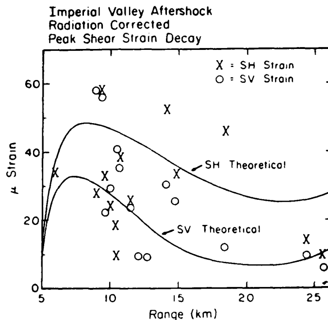
Figure 5. The decay of peak shear strain near to the Imperial Valley aftershock.
