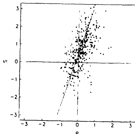
Figure 14. Correlation of the S and P station correction values derived in this study. The 3:1 scaling predicts a d\ln(v_p)/d\ln(v_s) of 1.7.
