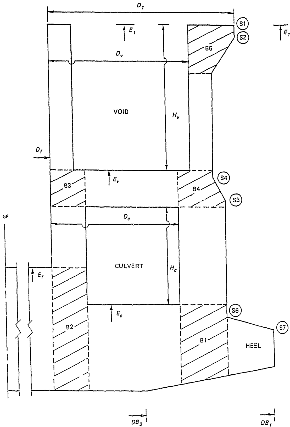
Figure 13. Type 33 monolith
