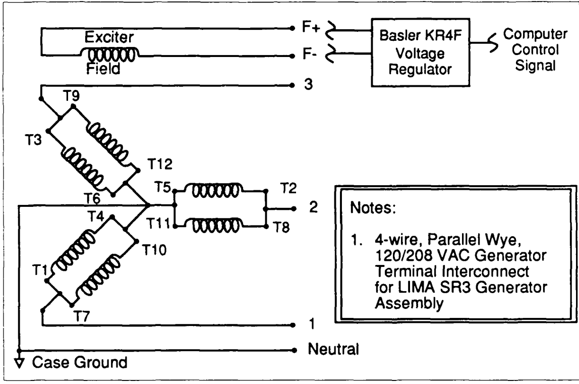
Figure 4. Generator Re-strap
