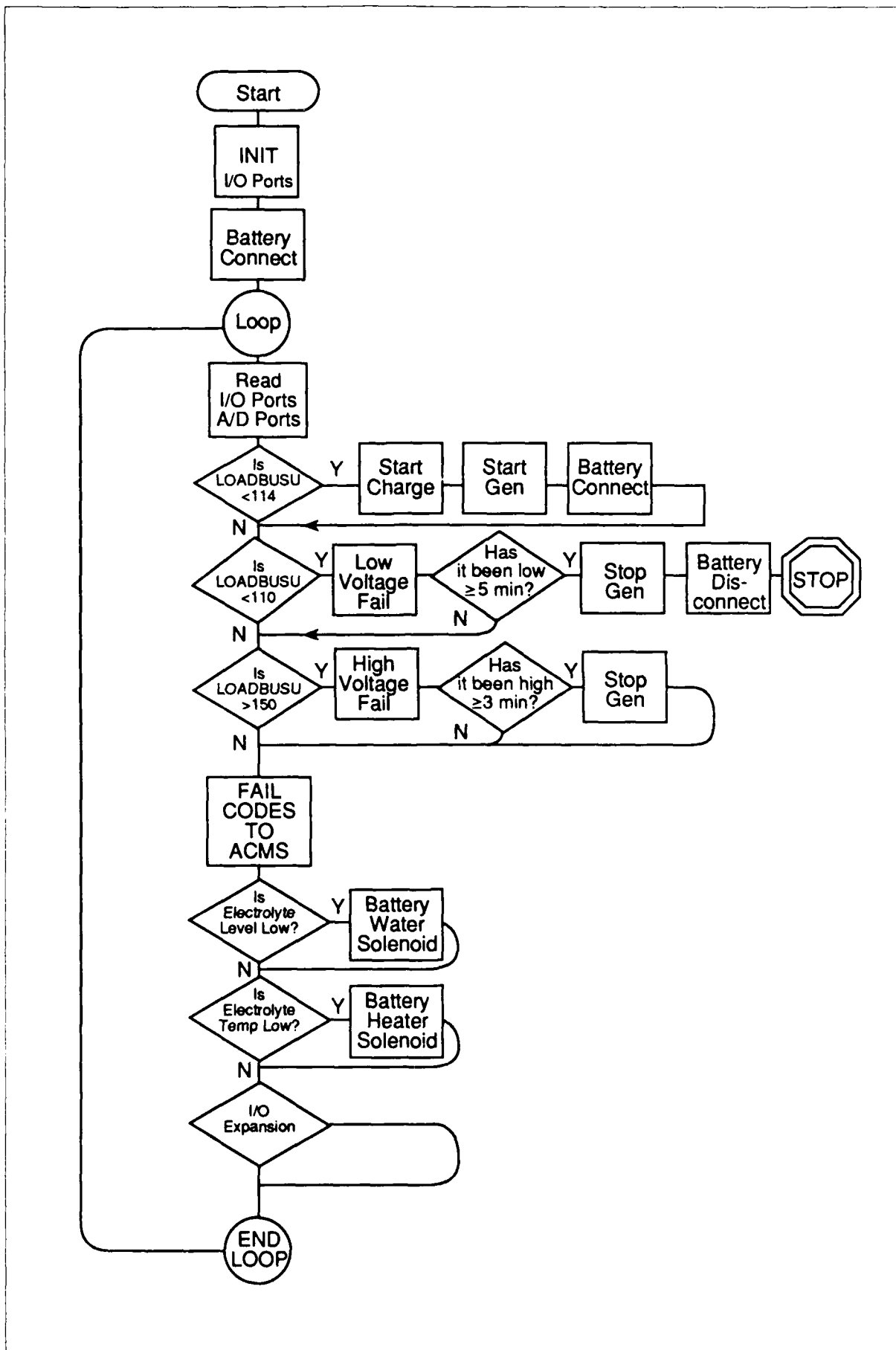
Figure 7. PSM Flowchart
