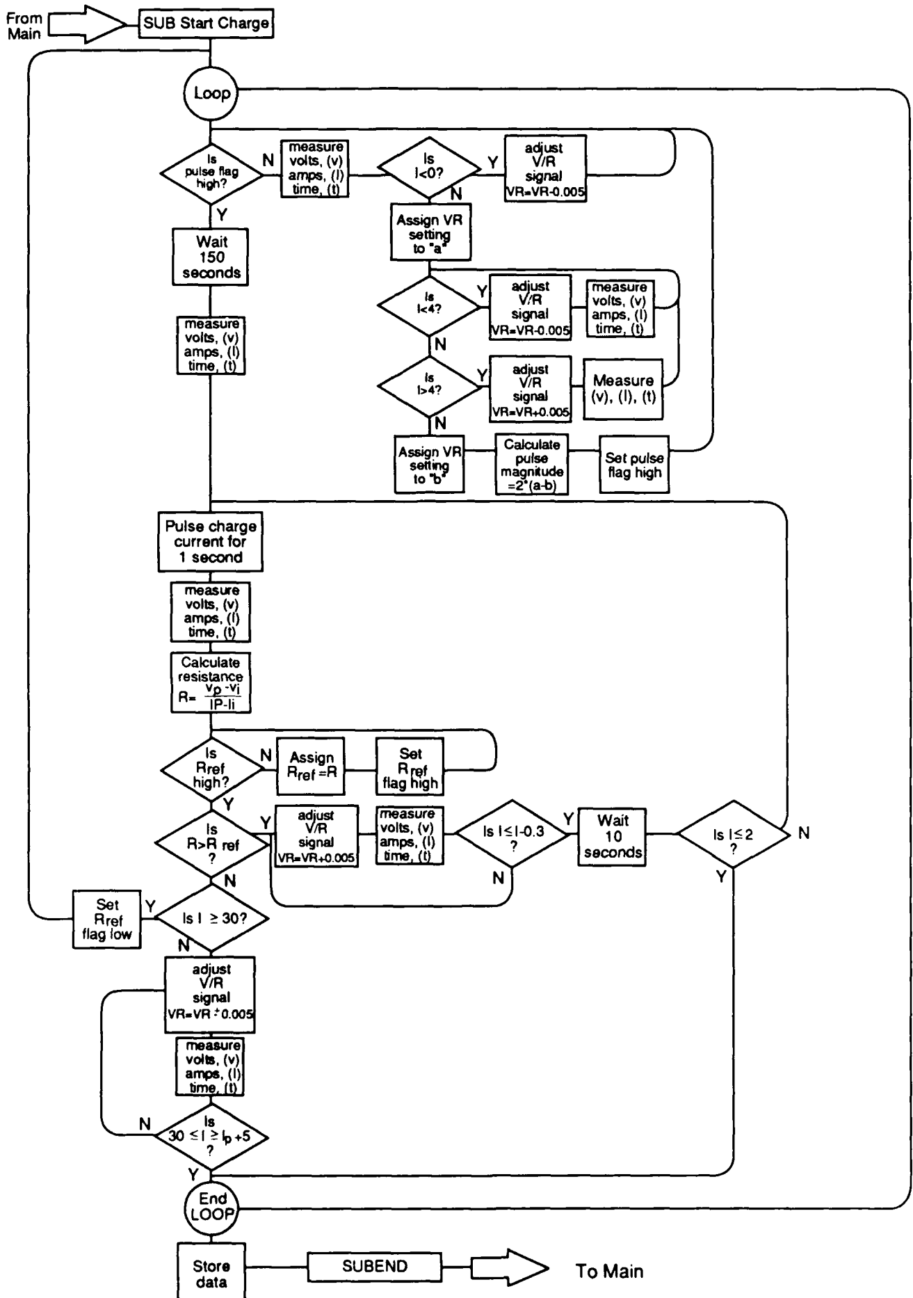
Figure 8. Charge Algorithm Flowchart
