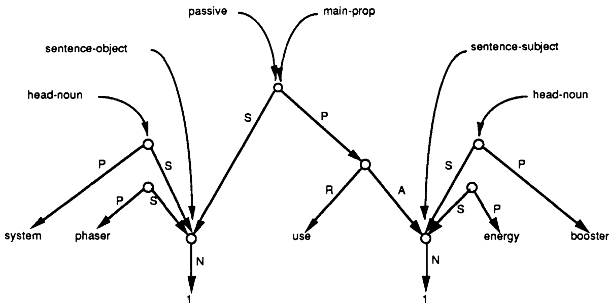
Figure 2. Example of ACT semantic network structure for the content of the sentence The energy booster is used by the phaser system . The arrows labelled with S, P, R, A, and N are links in the ACT structure, while the curved arrows represent TAGS specifying surface-structure information about the parts of the semantic structure.
