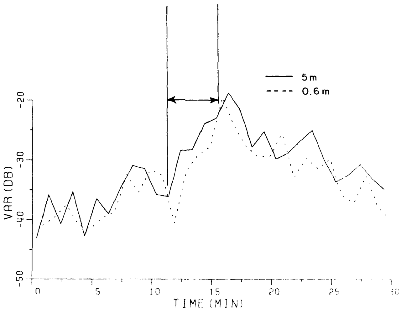
Figure 12. Enhanced large aperture scintillation during onset of precipitation fading.
