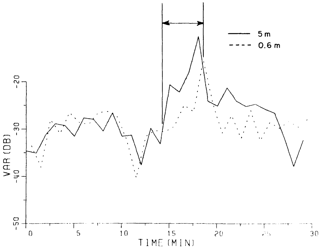
Figure 14. Enhanced large aperture scintillation during onset of precipitation fading.
