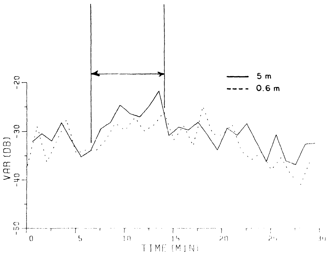
Figure 13. Enhanced large aperture scintillation during onset of precipitation fading.
