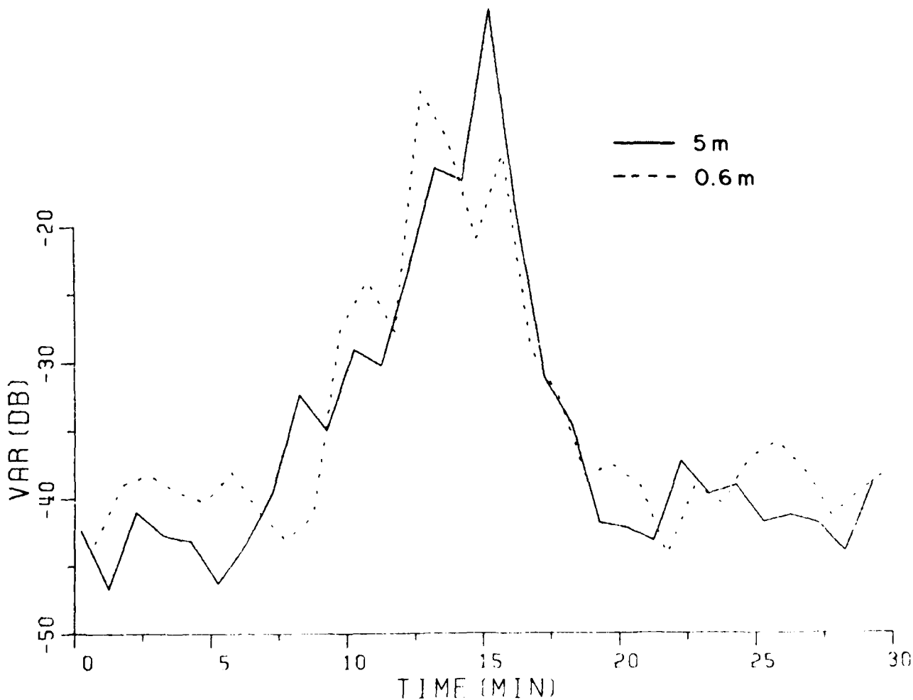
Figure 16. Variance behavior during a precipitation fade event.
