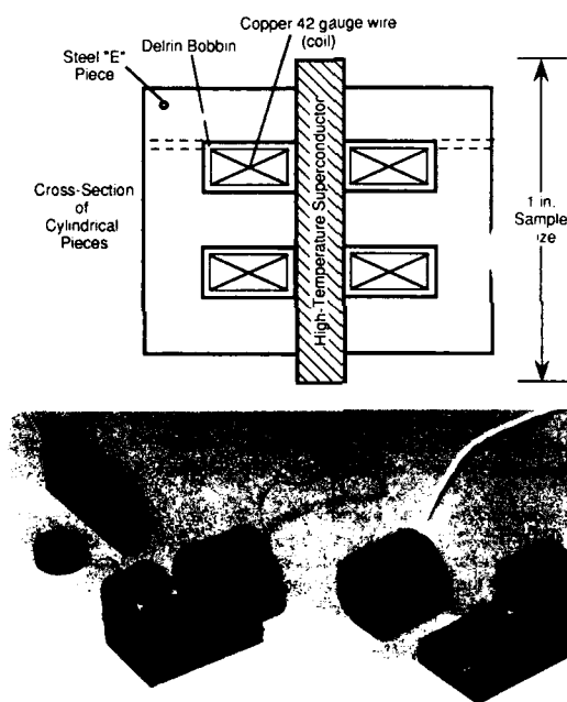
Figure 5. Sending and Receiving Coil with Sample
