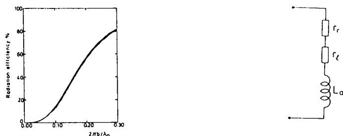
Figure 1 Efficiency of copper loop antenna Figure 2 Equivalent circuit for loop antenna
