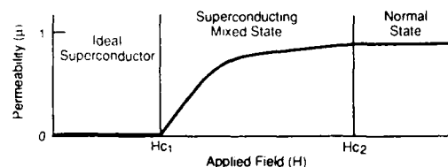
Figure 2. Typical Magnetization Curve for a Type II Superconductor
