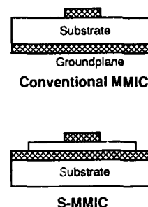
Figure 3. Geometries for standard MMIC (top) and Superconducting MMIC (bottom). In conventional MMIC the substrate material serves as the dielectric for wave propagation. Substrates are typically 0.5 mm thick. In the superconducting version, the groundplane is deposited on top of the substrate. Wave propagation is through a deposited thin film, typically 0.5 microns thick.
