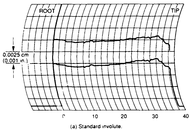
(a) Standard involute.
