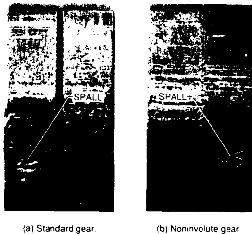
Fig. 6. Typical fatigue spall
