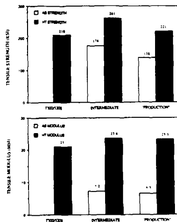
FIG. 4. PBZT/FX 3369 MC FIBER TENSILE PROPERTIES vs TPA/EPOXY UNI-COMPOSITE
