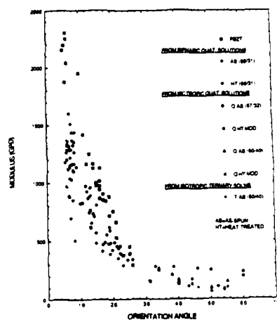
FIG. 3. MODULUS - ORIENTATION ANGLE RELATIONSHIP OF PBZT & MC'S
