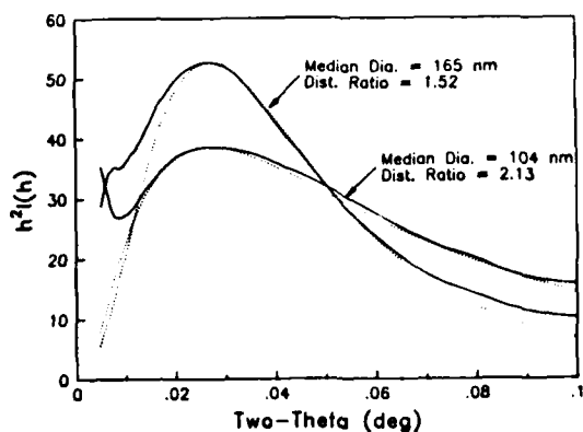
Figure 7 - Fitted Invariants for Blends
