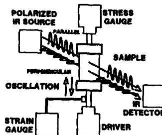
Fig. 1. Schematic representation of a DIRLD spectrometer.
