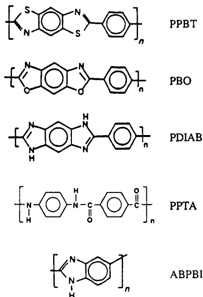
Figure 1. Chemical structures of PPBT, PBO, PDIAB, PPTA, and ABPBI.
