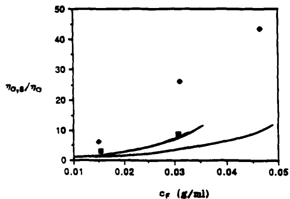
FIGURE 4: Ratios of blend to rod viscosities as a function of flexible chain concentration c_F . Points denote experimentally determined values, with symbols denoting blend compositions as in FIGURE 1. Lines denote viscosity ratios calculated by equation 7, as described in text. Upper line; blends with c_R = 0.043\text{ g/ml} . Lower line; blends with c_R = 0.028\text{ g/ml} .
