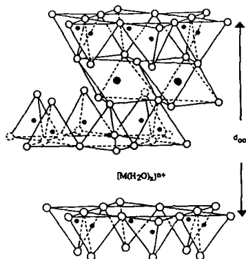
Figure 1. Idealized structure of a mica-type silicate.
