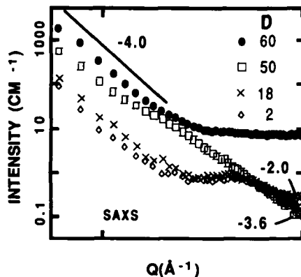
Fig. 7. SAXS data for the series of polymer-toughened glasses shown in Fig. 6.
