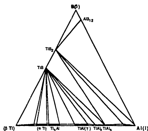
Fig. 5 Calculated phase equilibria for ternary system Ti-Al-B at 1100^\circ\text{C} .
