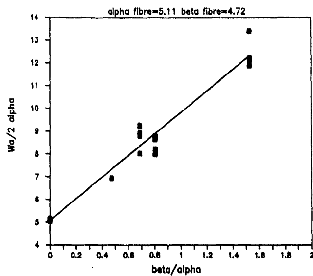
Figure 4 W_a/2\alpha_1 versus \beta/\alpha and best fit straight line for fibre B (controlled surface)
