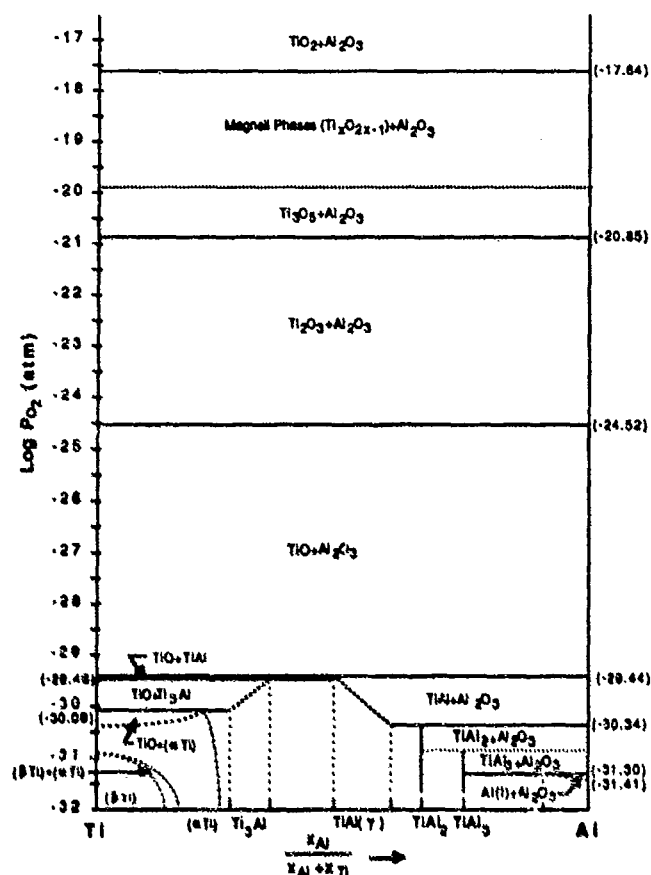
Fig. 2 Stability diagram for ternary system Ti-Al-O at 1100° C.
