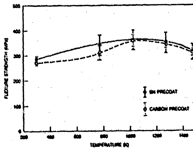
Fig. 5. High temperature flexure strengths for Nicelon/SiC composites with ~ 0.2 μm carbon and BN interface coating.
