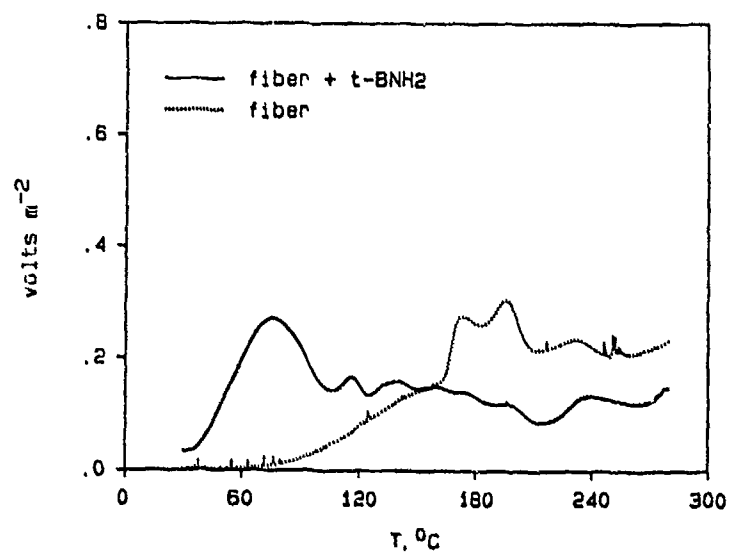
Figure 2. Thermal desorption from silicon carbide fiber after oxidative plasma treatment. Dotted curve denotes evolution from fiber without probe. Solid line shows evolution after injection of t -butylamine.
