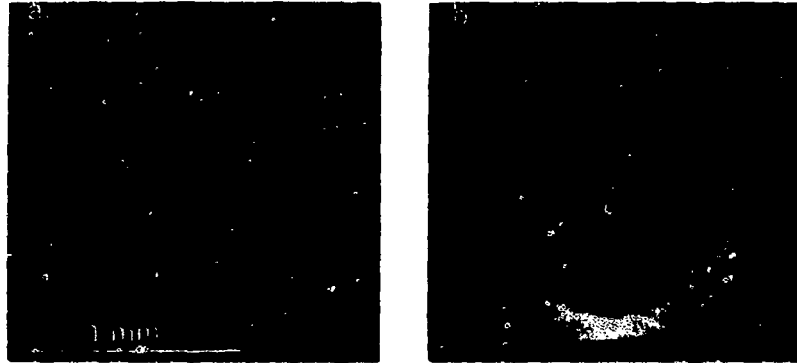
Figure 1. Micrographs of a 98 \mu\text{m} epoxy coating being subjected to Vickers indentation. (a) P = 15 \text{ N} , (b) P = 30 \text{ N} .
