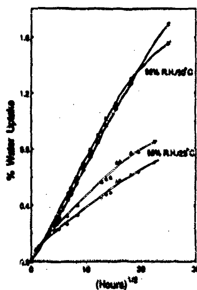
Figure 3. Water uptake for cured epoxy resin
