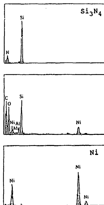
Figure 1 X-ray energy dispersive spectra of \text{Si}_3\text{N}_4 , amorphous, and Ni
