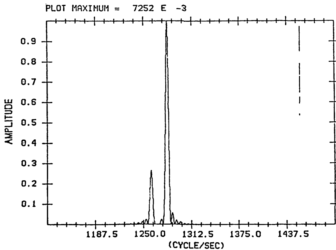
Figure 2. FFT Recovered PSD of Synthetic Interferogram.
