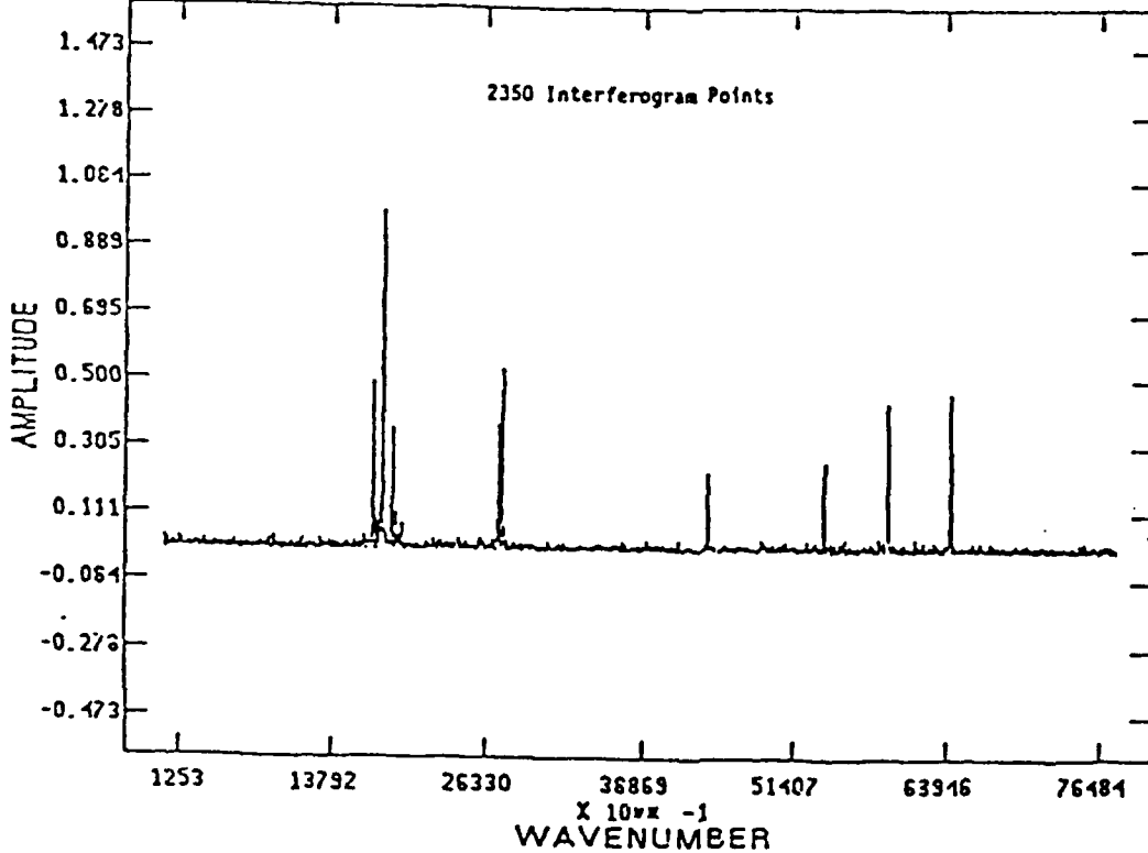
Figure 17. LABCEDE Interferogram Recovered with FFT.
