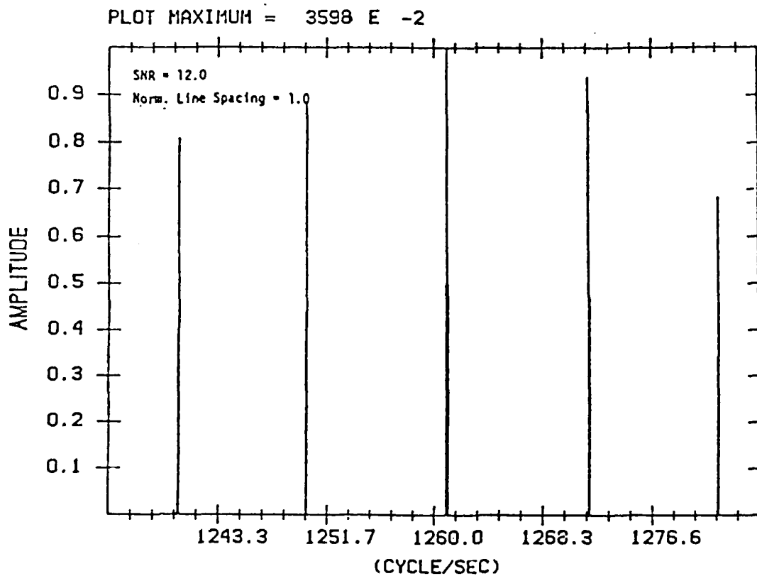
Figure 11. Five Equal Strength Lines Recovered with MEM and Integrated.
