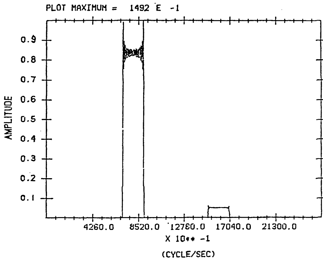
Figure 12. Two unequal Rectangles Recovered with FFT.
