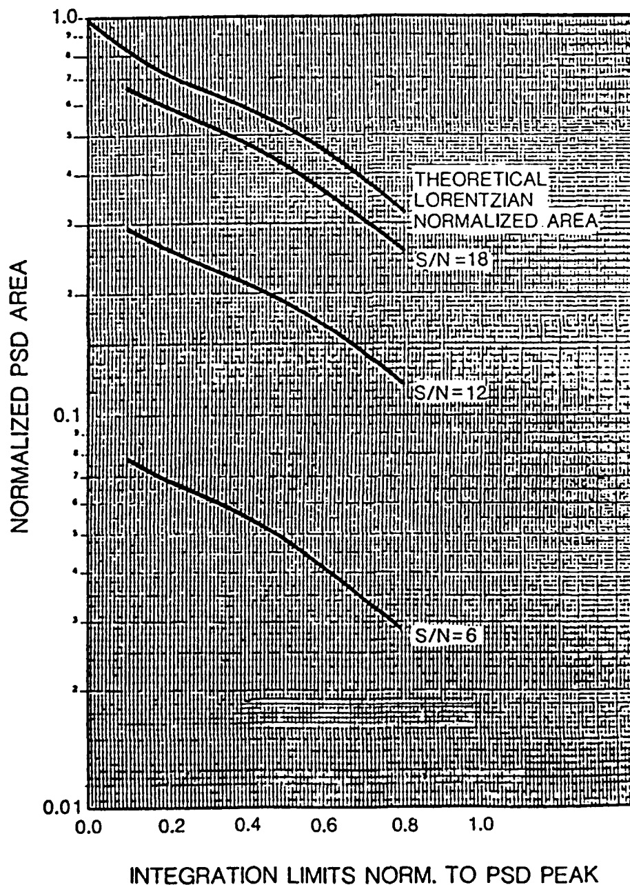
Figure 5. MEM Recovered PSD Area.
