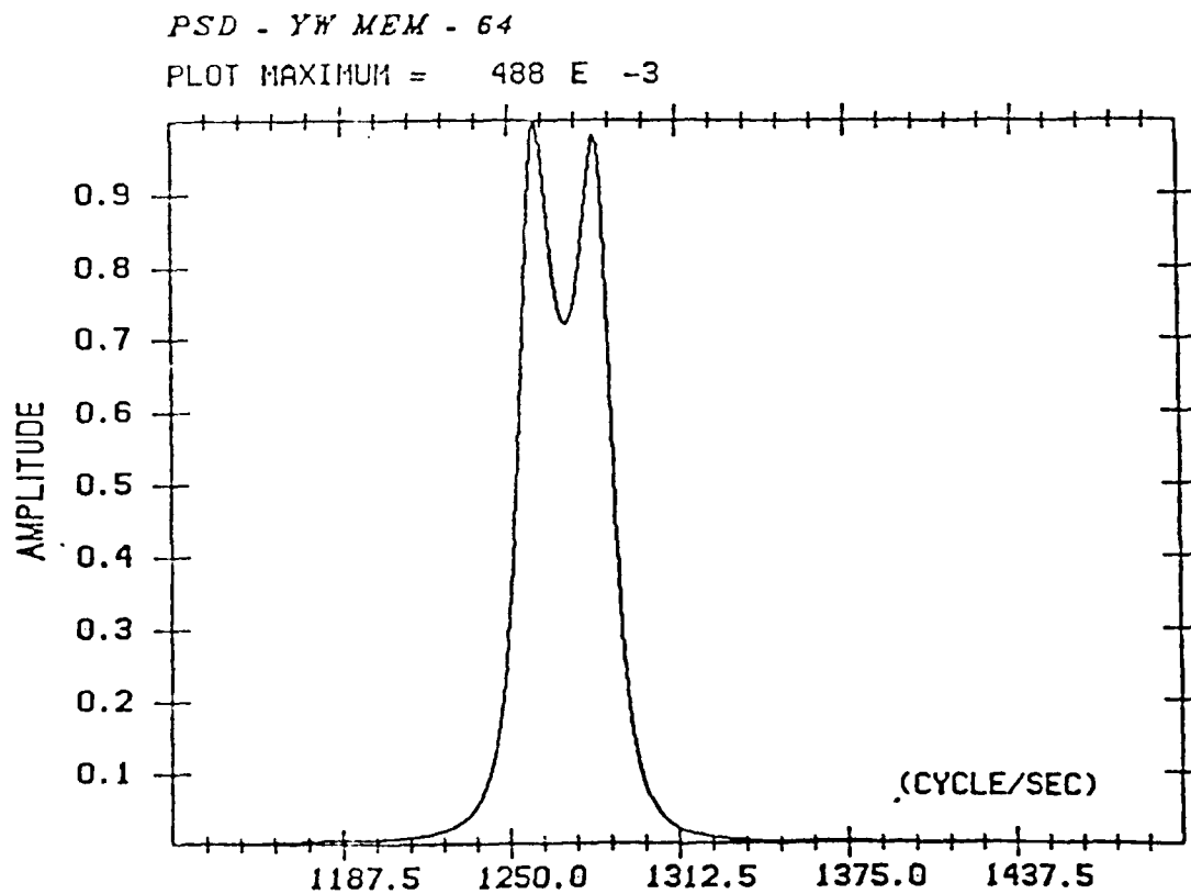
Figure 4. Recovered PSD of Synthetic Interferogram with Y-W MEM.
