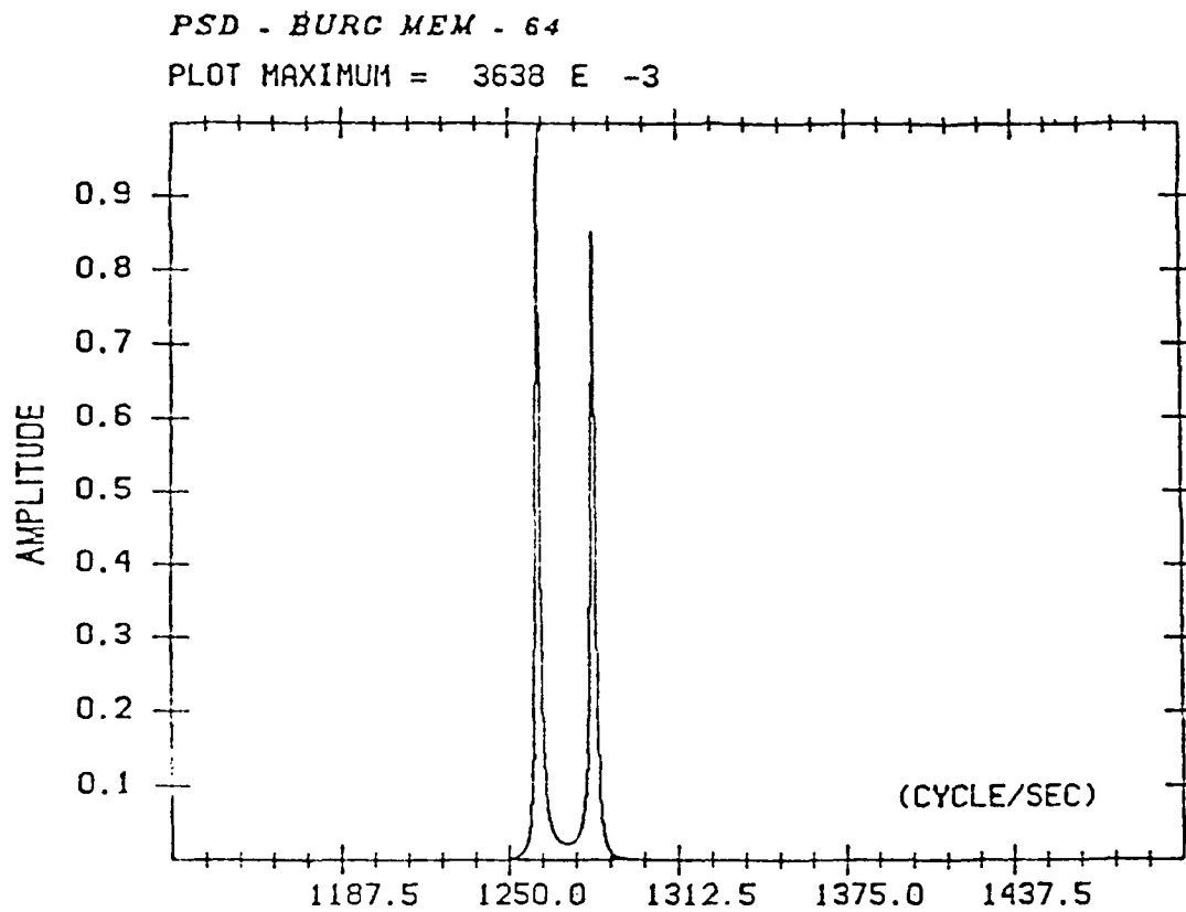
Figure 3. Recovered PSD of Synthetic Interferogram with Burg MEM.
