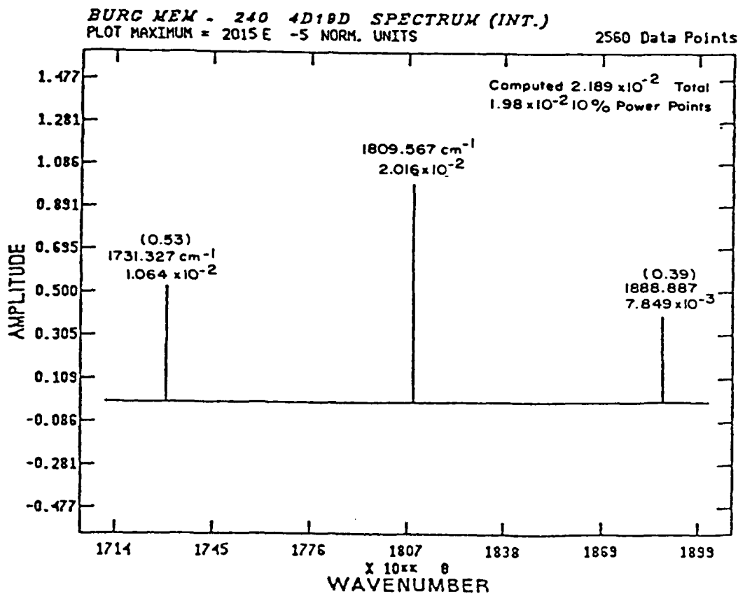
Figure 22. 600 Points of LABCEDE Interferogram Recovered with MEM and Integrated - Band 1.
