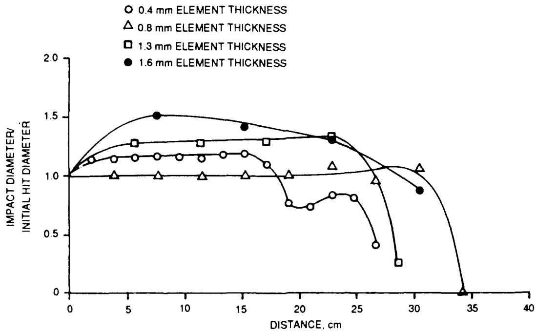
FIGURE 12. A Comparison of Normalized Impact Diameter Profiles for Different Target Sizes (1.7 km/s Initial Velocity).
