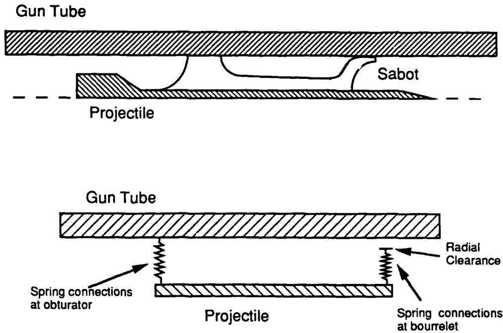
Figure 3. Simple Balloting Model for Gun Tube/Projectile Interaction.
