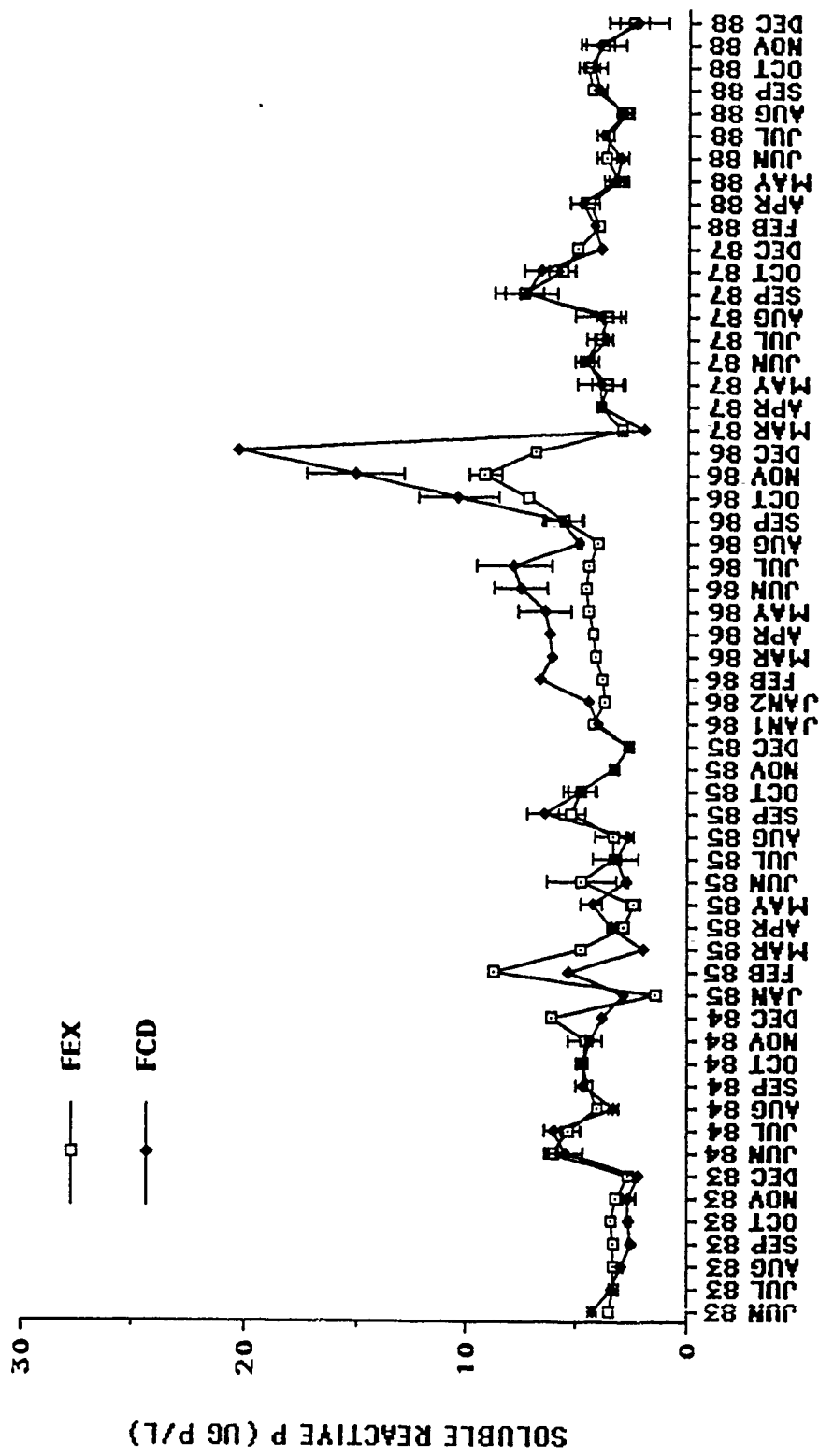
FIGURE 1.10 MEAN SOLUBLE REACTIVE PHOSPHORUS CONCENTRATION (+S.E.) FOR EACH 28 DAY PERIOD FOR EXPERIMENTAL (FEX) AND CONTROL (FCD) SITES, 1983-1988.
