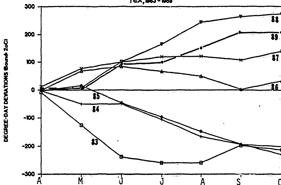
FIGURE 4.8A DEVIATIONS IN MEAN VALUES, DEGREE-DAYS fex, 1983 - 1989
