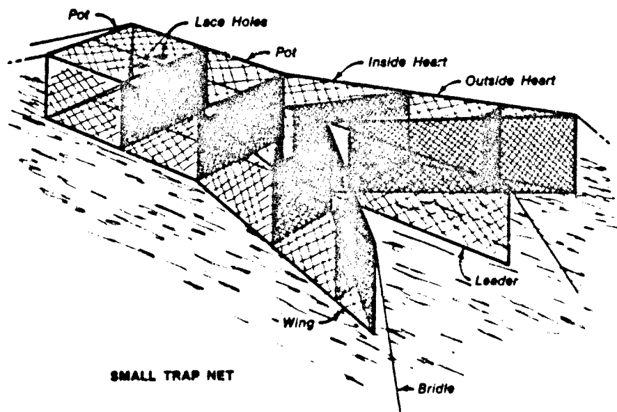
Figure 26. Hoop net and trap net designs (from Nielsen and Johnson 1983)
