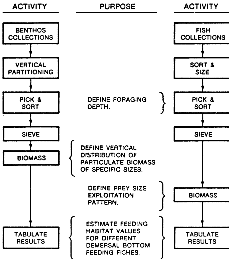
Figure 28. Flowchart for use of the BRAT
