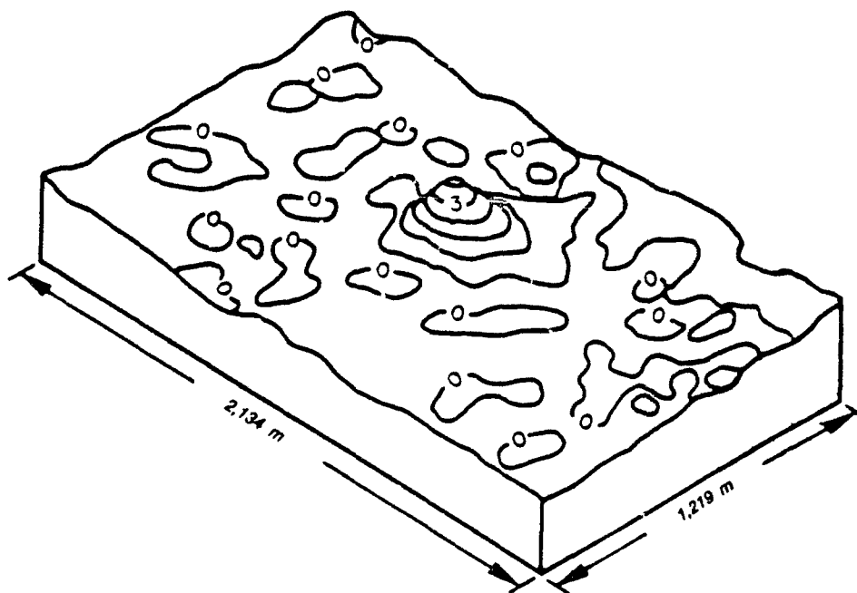
Figure 2. Contours of elevation differences due to disposal operations at the Dam Neck disposal site (contours in metres)
