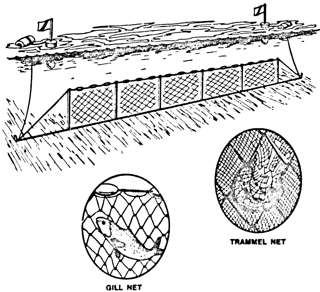
Figure 25. Gill net and trammel net (from Nielsen and Johnson 1983)
