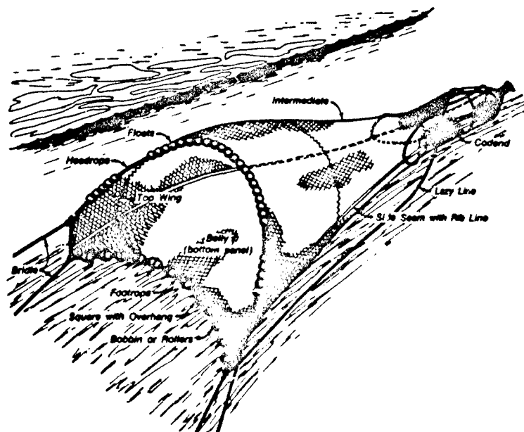
a. Otter trawl (from Nielsen and Johnson 1983)
