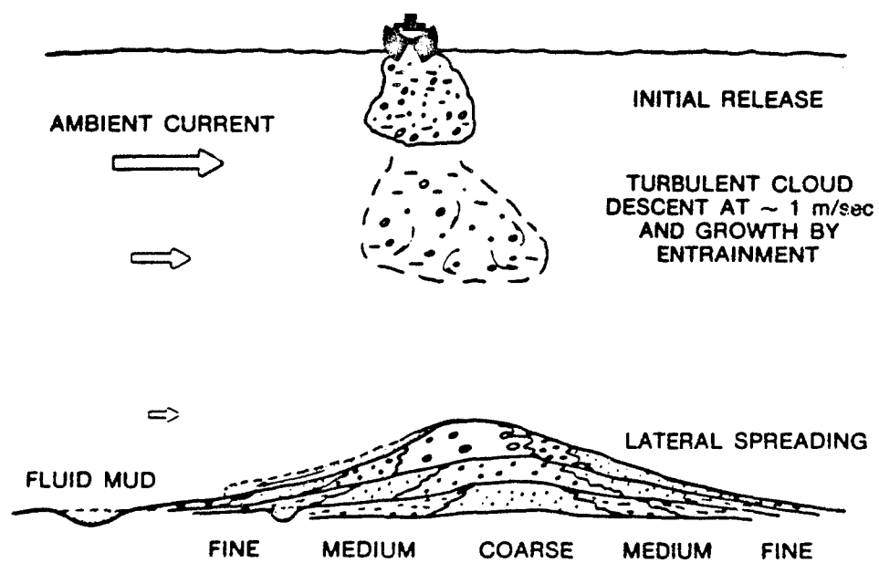
Figure 11. Radial sorting of disposal material
