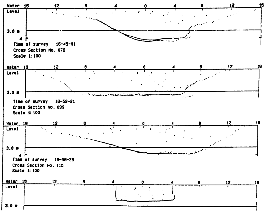
Figure 5. Sample cross sections from a scanning profiler (after Ulvertech America, Inc. 1985)
