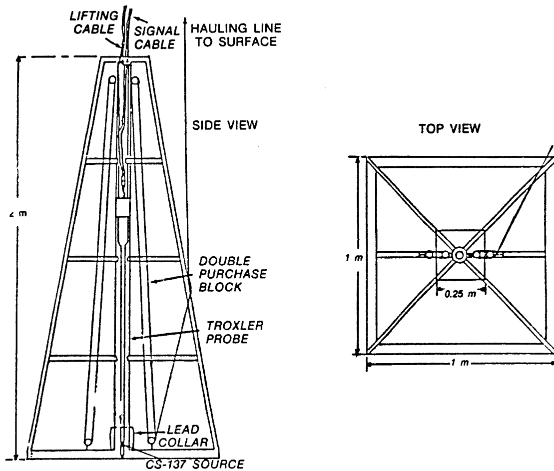
Figure 19. Nuclear density probe (from Morton, Stewart, and Germano 1984)
