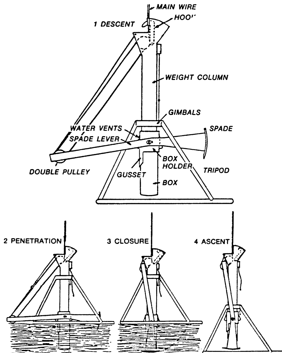
Figure 15. Box corer (from Lee and Clausner 1979)
