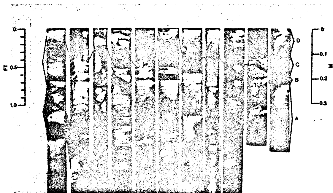
Figure 14. Dam Neck disposal mound core x-rays. Native (A), early disposal (B), and recent disposal materials (undisturbed, C, and reworked, D) are easier to distinguish with radiographs than with visual inspections
