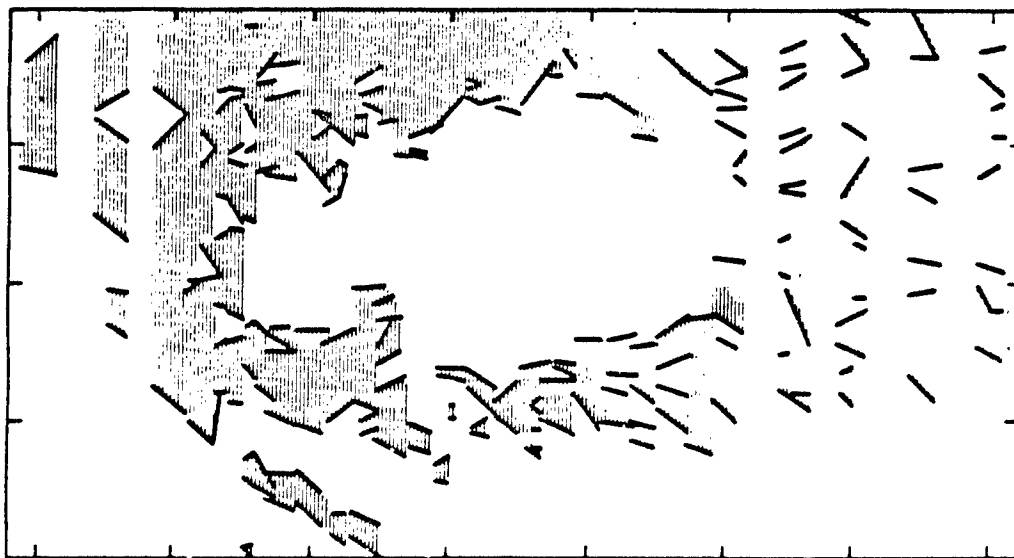
Figure 7. Predisposal and postdisposal maps of the Dam Neck disposal site produced from side-scan sonar records. The large low-backscatter area in the center of the postdisposal map represents the footprint of the disposal mound. Smaller areas scattered farther afield represent thin deposits of the finer-grained material
