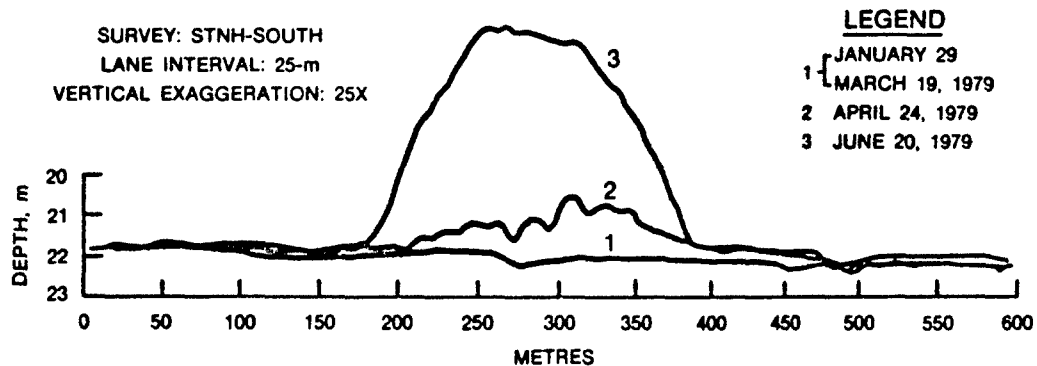
Figure 1. Bathymetric cross section from the Stanford New Haven disposal site capping operation in Long Island Sound (from Science Applications, Inc. 1985)
