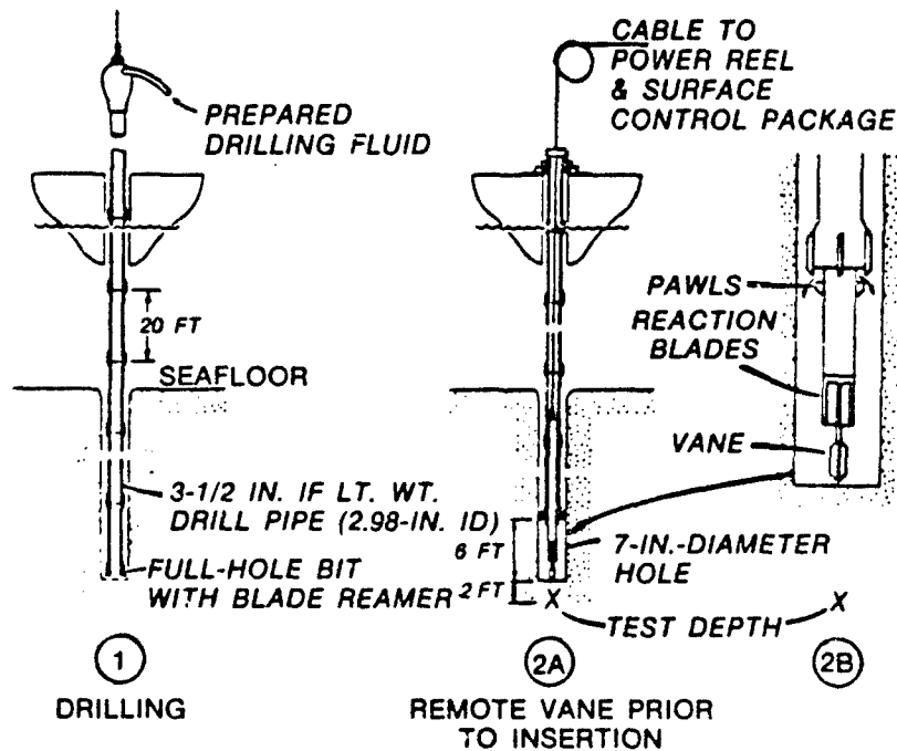
Figure 21. Field vane shear device on a wireline
