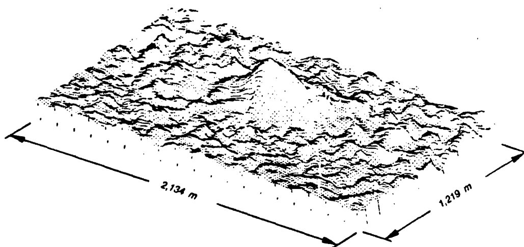
Figure 3. Three-dimensional plot of the Dam Neck disposal site (note mound in the center)
