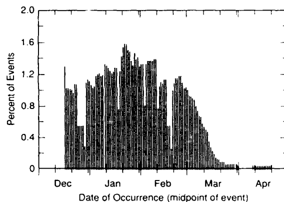
b. Upland streams.
