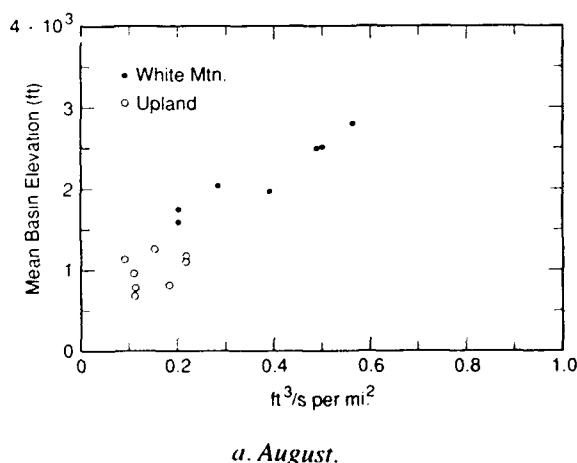
Figure 8. Discharge per square mile versus mean basin elevation for 3-day January and August events on White Mountain and Upland Section streams.
