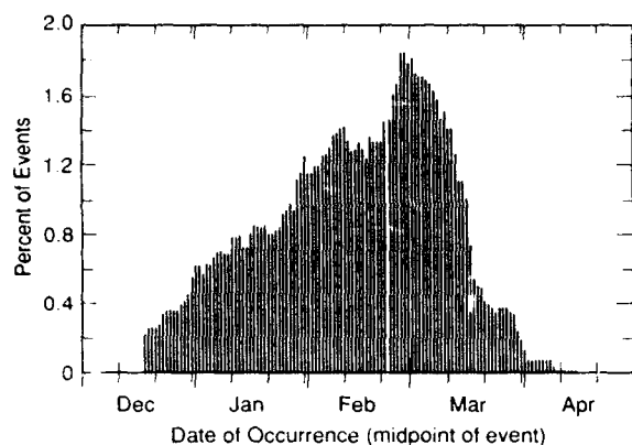
a. White Mountain streams.
