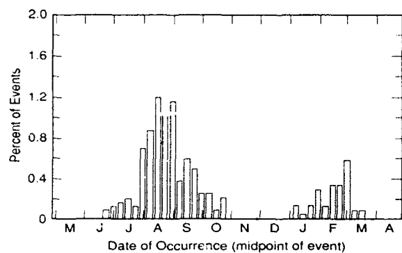
a. White Mountain streams.
