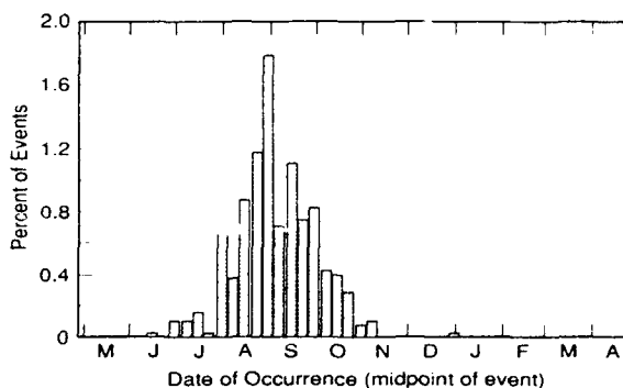
b. Upland streams.
