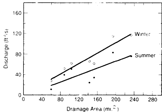
1. White Mountain streams.
