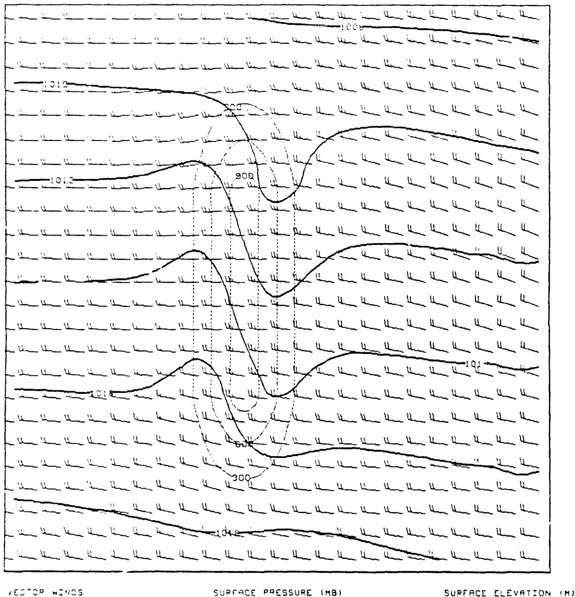
Fig. 24. Horizontal plot of FGM domain at 12 h for simulation with weak diffusion on temperature ( \sigma_s = 0.80 ). Solid contours give sea-level pressure (in mb), thin dashed contours are for surface topography (in m) of the mountain ridge, and boundary layer winds (one full barb represents 10 \text{ m s}^{-1} ) are plotted at each grid point.
