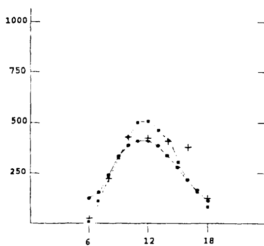
Fig. 35. Various fluxes for O'Neill case data from the one-dimensional version of the boundary-layer parameterization (solid line connecting dots), previous model (dashed line connecting squares), and observations (crosses).
