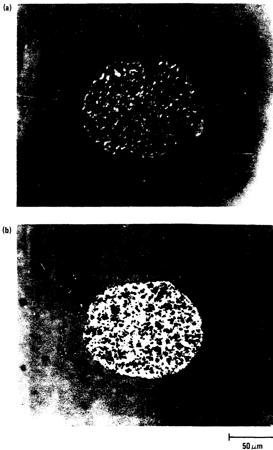
Fig. A-29. (a) The optical micrograph of the polished cross section of fiber calcined at 915^{\circ}\text{C} , 24 h showing finer grain size (polarized light; 400X; J_c = 1100 \text{ A/cm}^2 ); (b) unpolarized light to show a large amount of porosity (400X)
