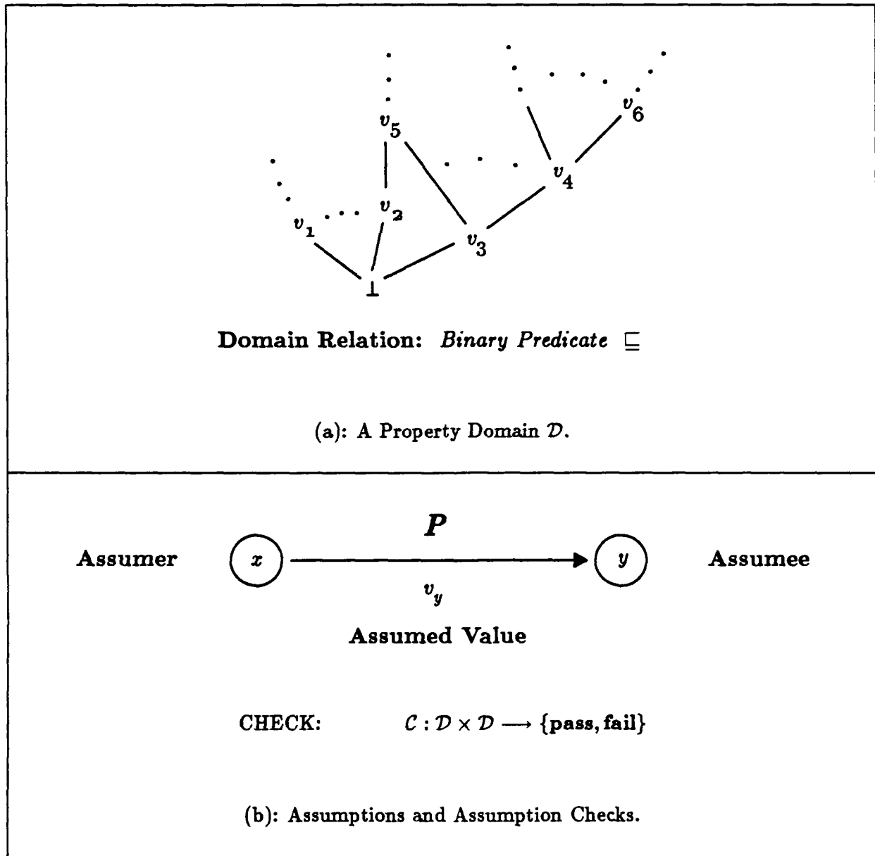
Figure 3.1: A general framework for Properties and Assumptions.
