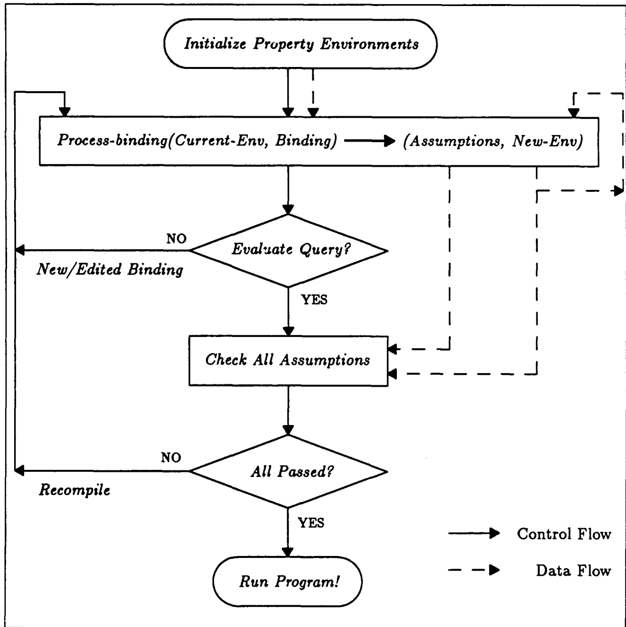
Figure 3.2: Overall Plan for Incremental Property Maintenance.
