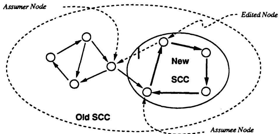
(b): Using the SCC Assumptions (Q) to detect Reduced SCCs.
