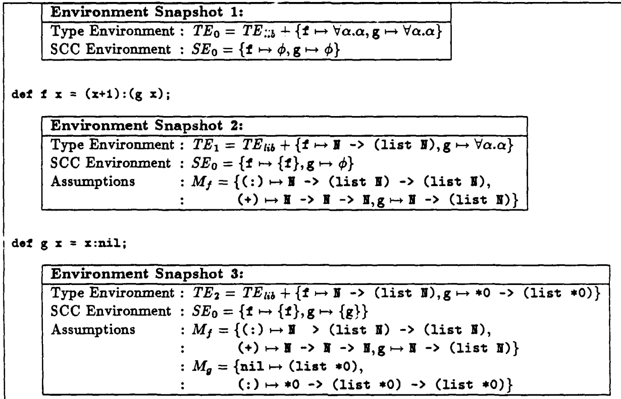
Figure 3.7: An Example to show Incremental Type Inference.
