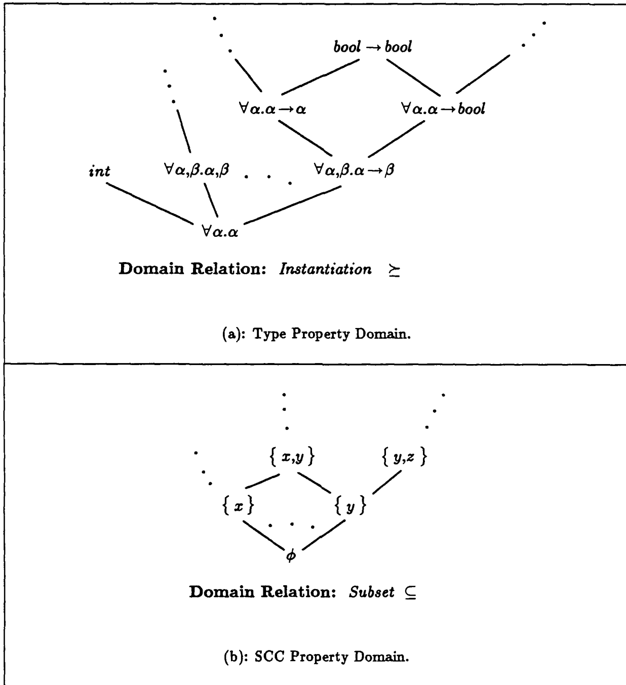
Figure 3.3: Compilation Properties used in Algorithm W_1 .
