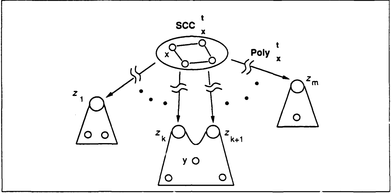
Figure 3.11: The Inductive Step in the Soundness Proof of Type Computation.
