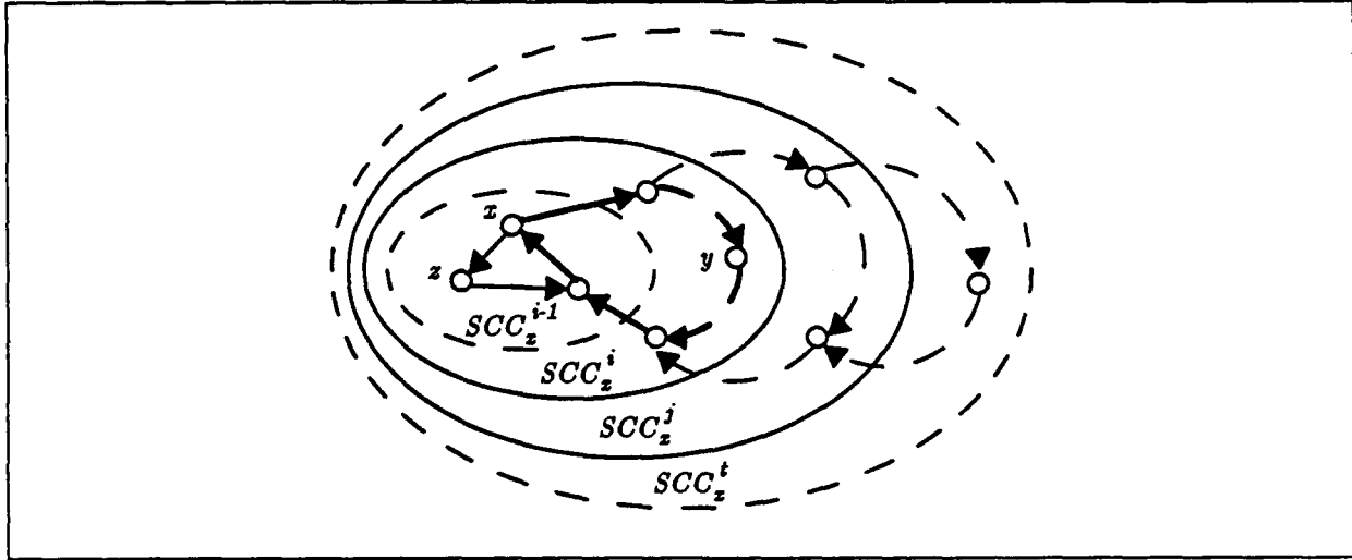
Figure 3.9: The Strongly Connected Components of x at various incremental stages.
