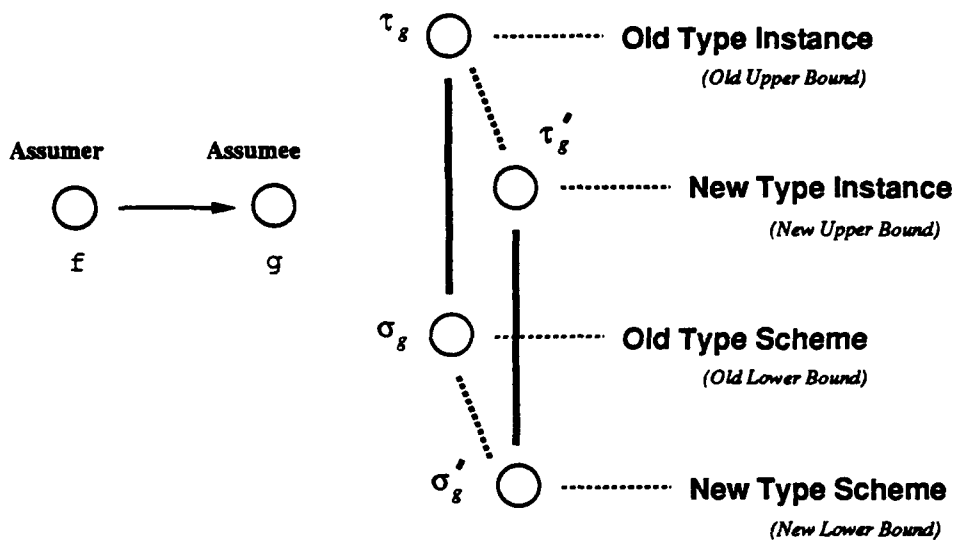
(a): Using the Lower Bound Assumptions (N) to detect Type Constraint Relaxation.
