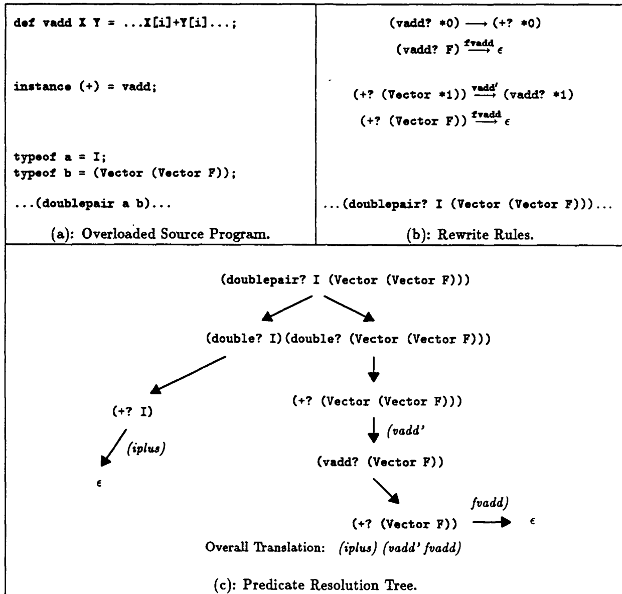
Figure 4.12: An Example of Overloading Resolution and Specialized Translation.
