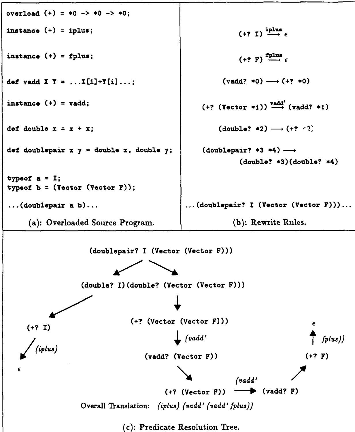
Figure 4.6: An Example of Overloading Resolution and Parameterized Translation.
