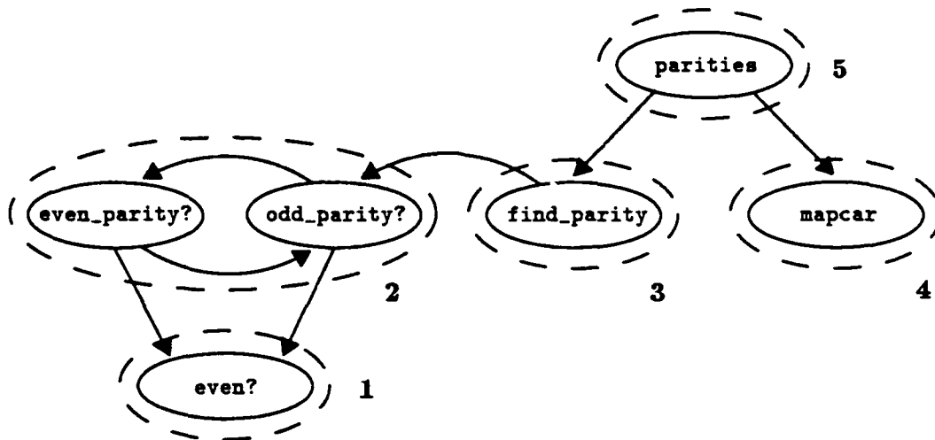
(b): Static Call Graph.
