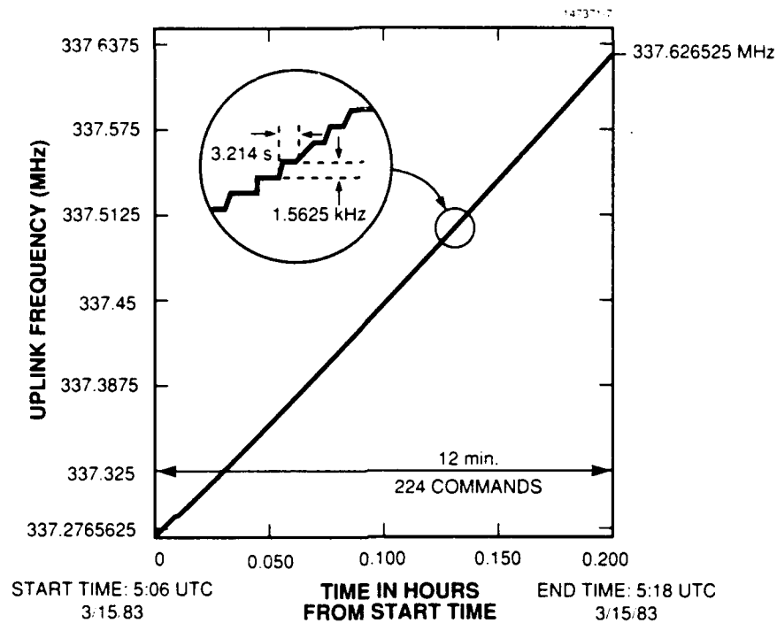
Figure 7. Received uplink frequency vs time, sample channel.
