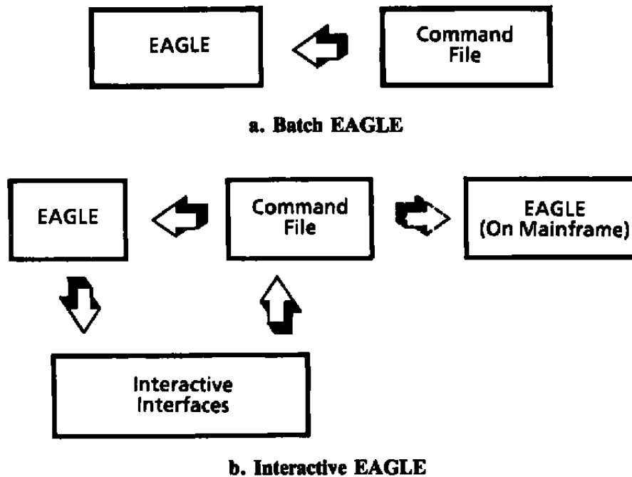
Figure 1. Data flow of batch and interactive EAGLE.
