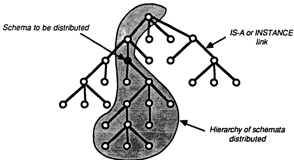
Figure 6-3: Hierarchical distribution example
