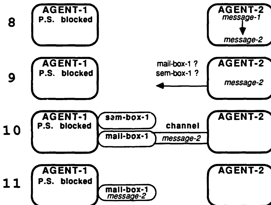
Figure 4-7: Message passing with blocking: step 3
