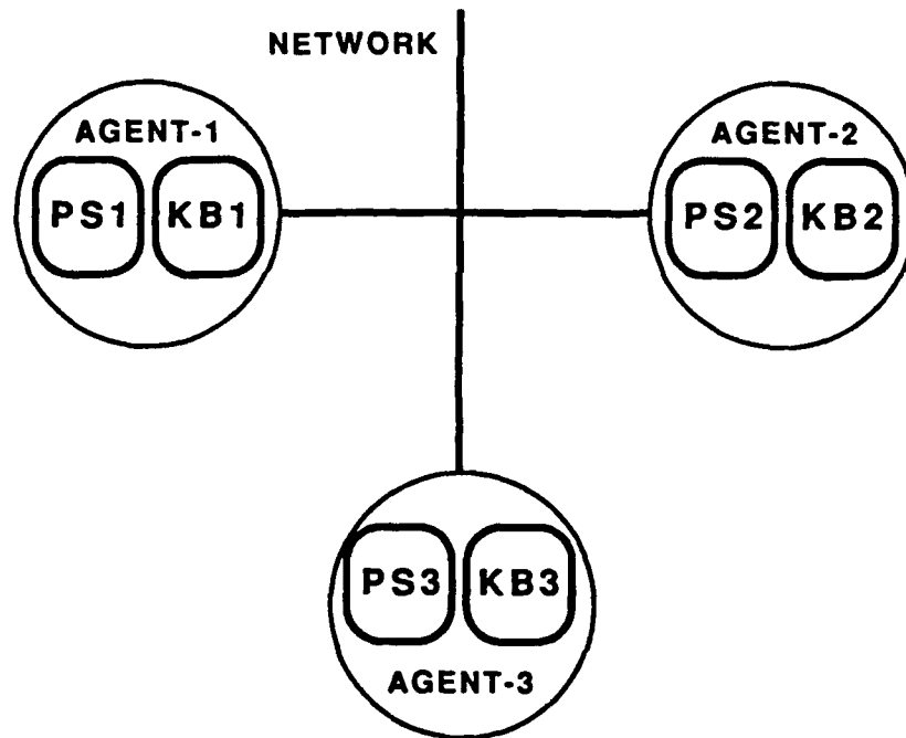
Figure 3-4: Decentralized system example
