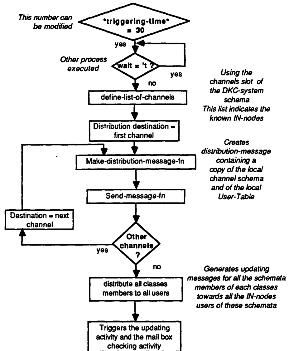
Figure 6-4: Distribution sequence for an EMN-node initialization
