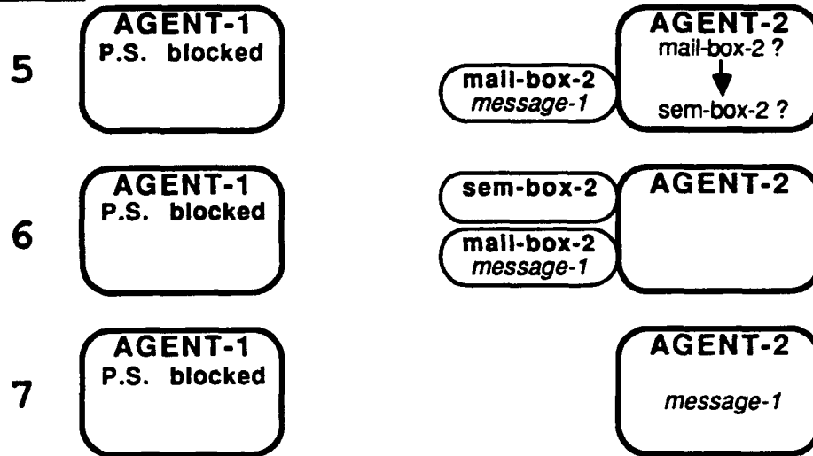
Figure 4-6: Message passing with blocking: step 2
