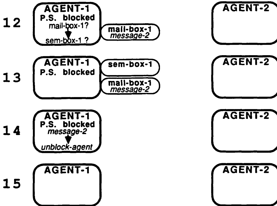
Figure 4-8: Message passing with blocking: step 4
