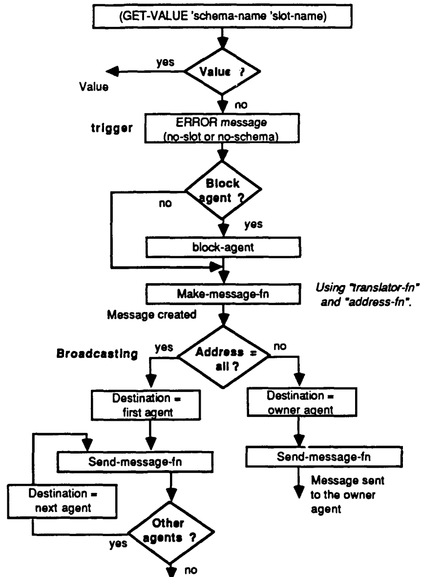
Figure 6-6: Message generation sequence
