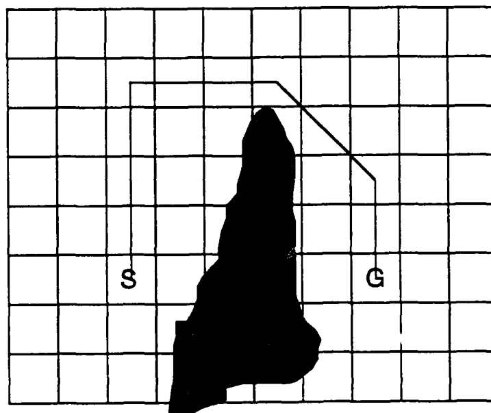
Figure 11: The Problem of Grid Bias
