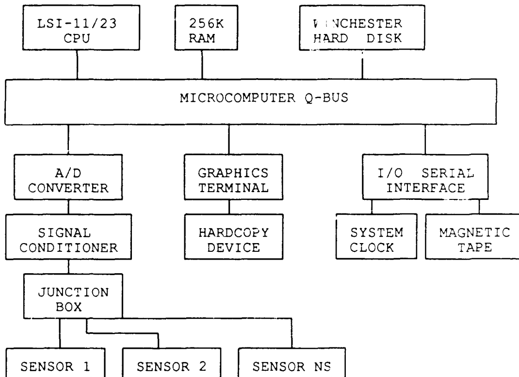
The diagram shows the Geophysical Data Acquisition System (GDAS) hardware flow chart. The "signal conditioner" module contains the preamplifier and filter electronics.
