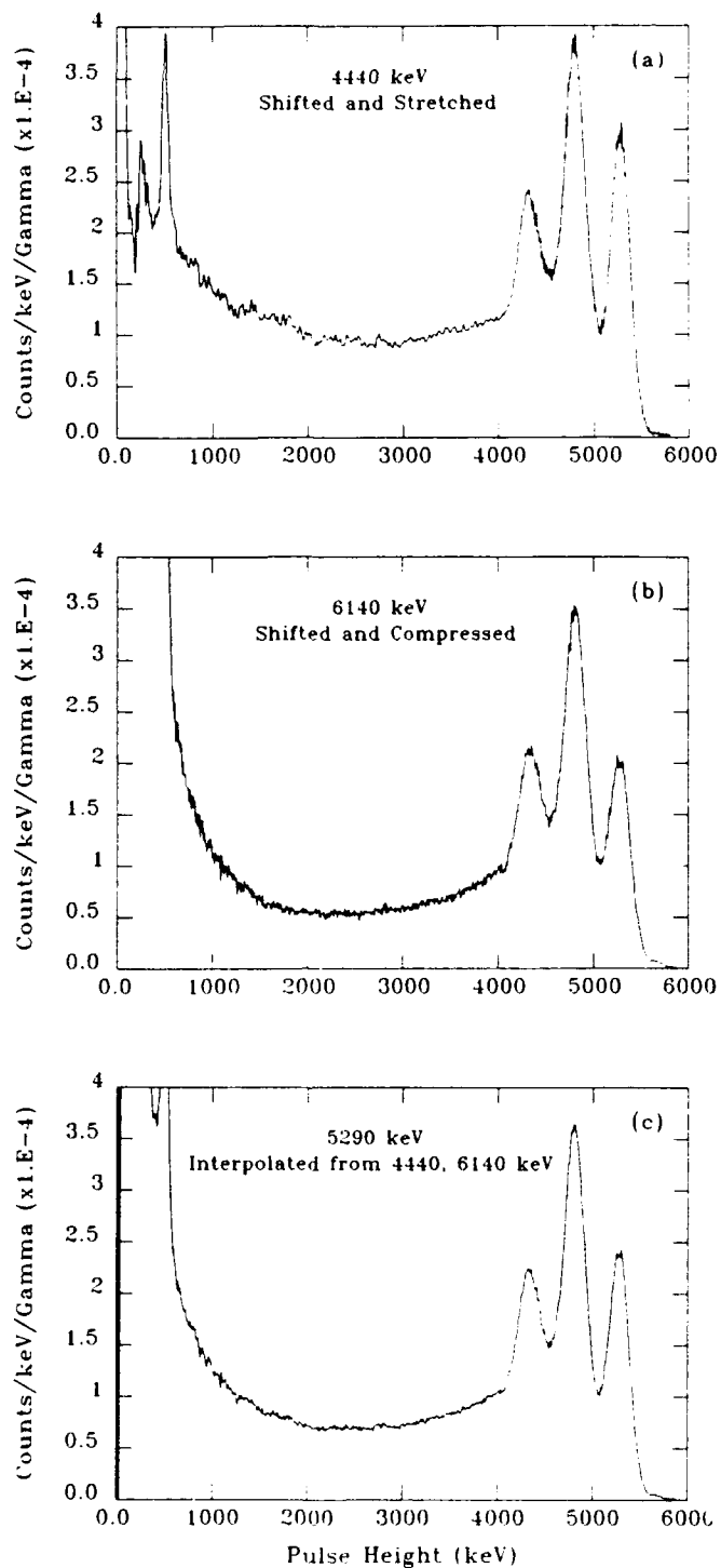
Figure 14. (a) Response function curve for the 2.54-cm x 2.54-cm BGO scintillation detector at E_\gamma = 4440 keV in which the pulse-height axis has been shifted and stretched to match the pulse-height axis for E_\gamma = 5290 keV. (b) Response function curve at E_\gamma = 6140 keV in which the pulse-height axis has been shifted and compressed to match the pulse-height axis for E_\gamma = 5290 keV. (c) Response function curve at E_\gamma = 5290 keV interpolated from the 4440- and 6140-keV response curves.
