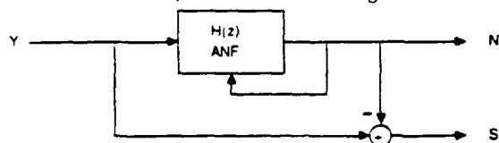
Figure 5 - Adaptive Line Enhancer
