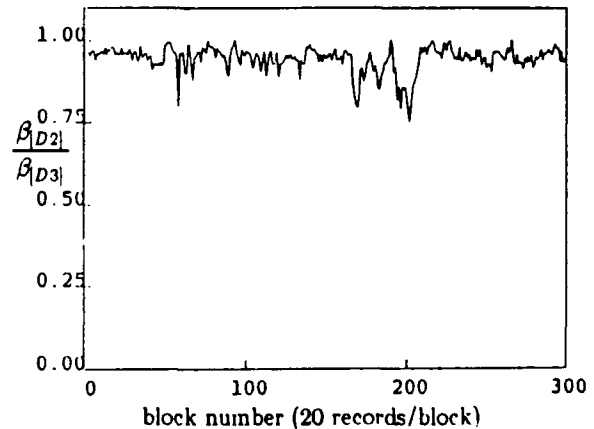
Figure 9 - Ratio of Power Levels between [D2] and [D3] for \alpha = 0.20
