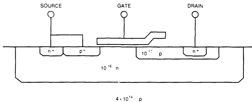
(b) HIGH VOLTAGE P-CHANNEL FET
