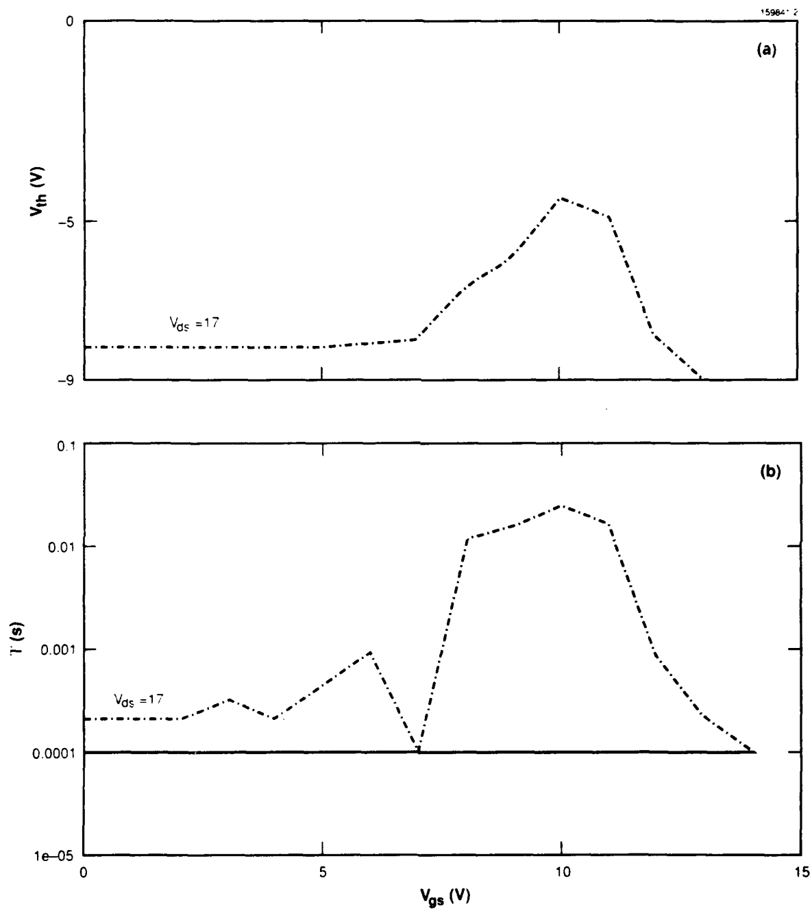
Figure 2. N-type stacked gate structure, 1:4 coupling, 2- \mu m gate length: (a) maximum threshold voltage and (b) writing time.
