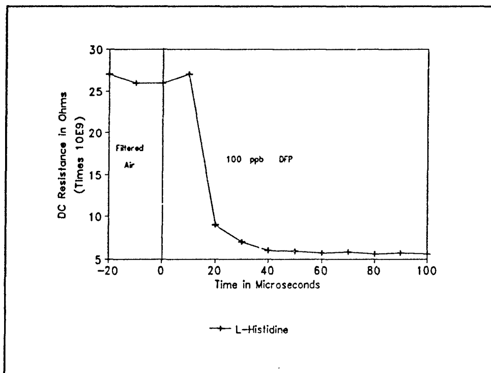
Figure 51. L-Histidine Dihydrochloride DC Resistance Change With Respect to Time due to a 100 ppb DFP Challenge at 30° C.
