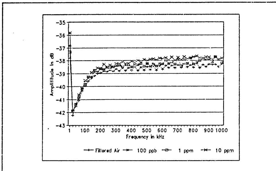
Figure 83. Copper Phthalocyanine Thin Film, 2000Å Thick, High-Frequency Response to DIMP Challenge Gas at 70° C.
