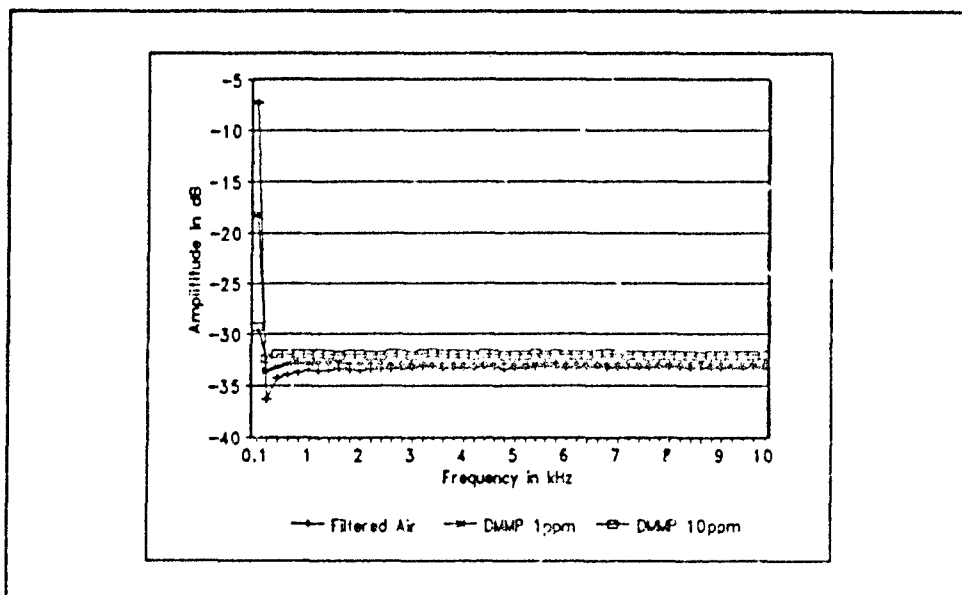
Figure 111. Copper Phthalocyanine Thin Film, 2000Å Thick, Low-Frequency Response to DMMP and DFP Challenge Gas at 30° C.
