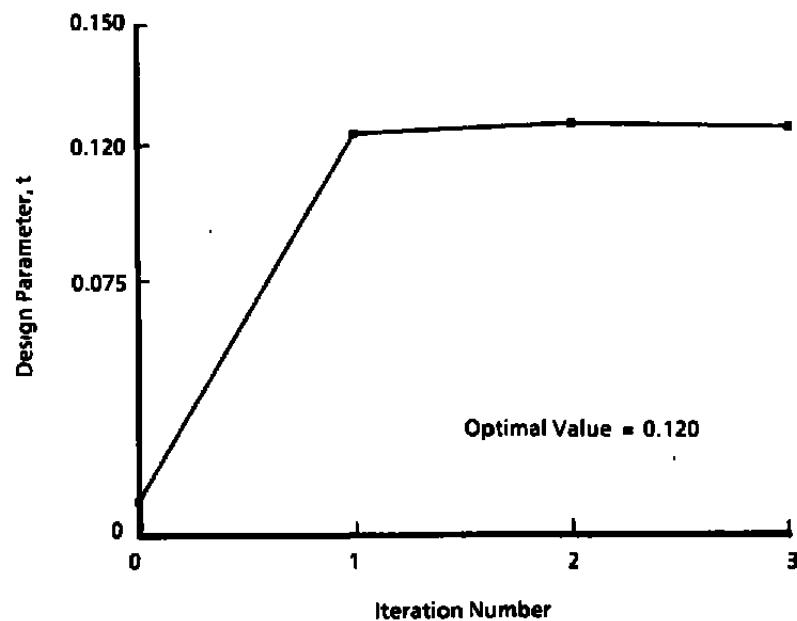
Figure 16. Viscous airfoil design parameter convergence.
