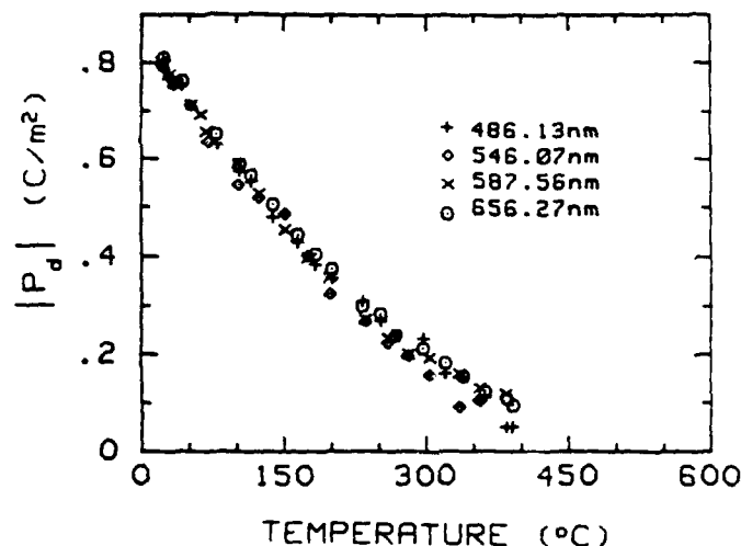
FIGURE 6 |P_d| as a function of temperature for .93(\text{Pb}_{0.99}\text{La}_{0.01})(\text{Mg}_{0.99}\text{Nb}_{0.01})\text{O}_3-.07\text{PbTiO}_3 calculated from n(T) data.
