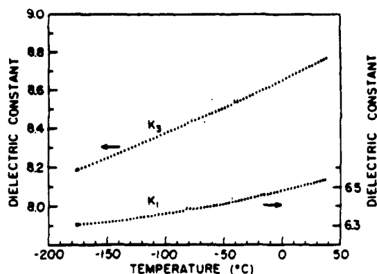
FIG. 2. Temperature dependence of dielectric constants K_3 ( \parallel [100] ) and K_1 ( \parallel [001] ) of \beta\text{-BaB}_2\text{O}_4 single crystal (frequency range 10^2 – 10^5 Hz).
