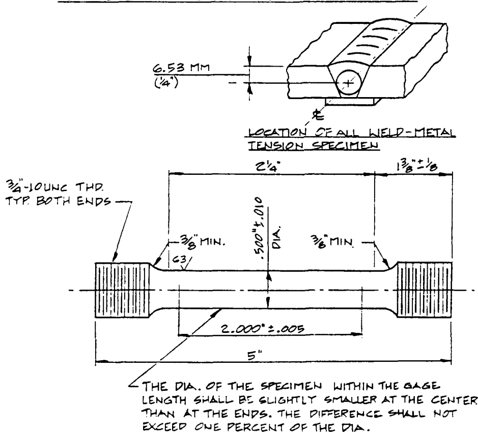
TEST PLATE SHOWING LOCATION OF TEST SPECIMENS
