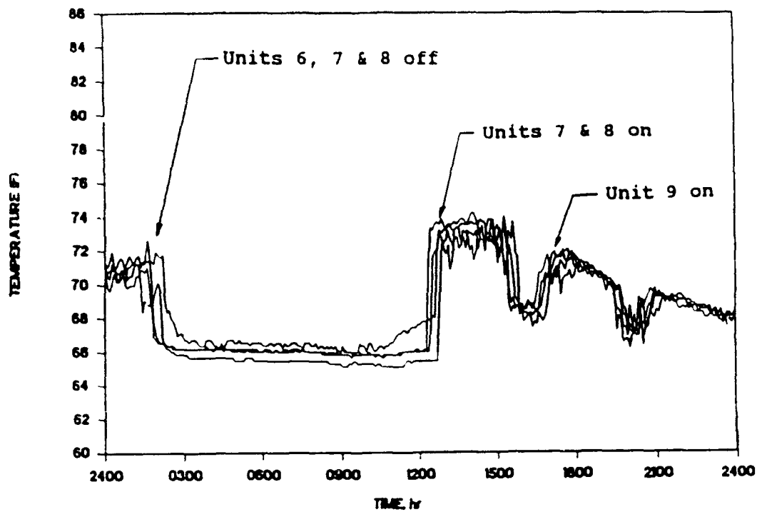
Figure 2. Temperatures recorded across the penstock and gatewell thermistors showing the typical effects of unit operations on the temperature recorded in slot 7B (27 July 1988).
