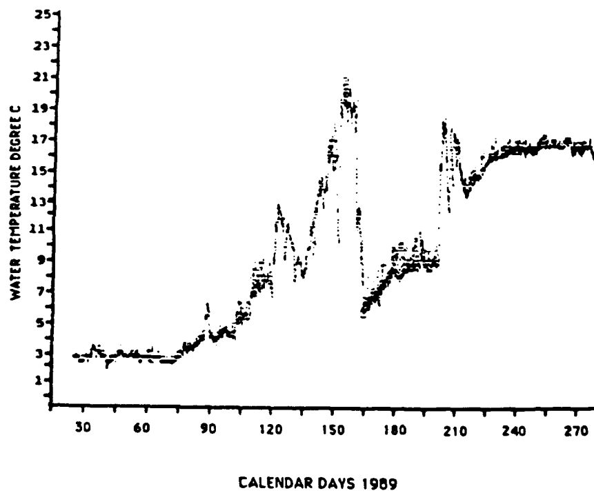
Figure 8. Inflow Temperature, 1989
