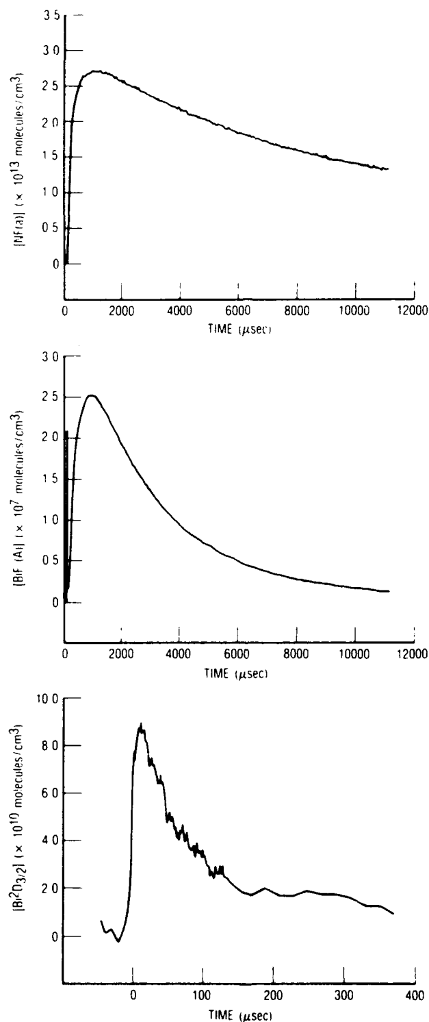
Fig. 8. Excited State Time Histories of NF(a^1\Delta) , BiF(A^1) , and Bi(^2D_{3/2}) . The Bi(^2D_{3/2}) trace was obtained from time-resolved absorption data. Reagent concentrations were [NF_2] = 1.5 \times 10^{15} , [Bi(CH_3)_3] = 2.2 \times 10^{15} , [H_2] = 1.1 \times 10^{15} , and [CO_2] = 5.0 \times 10^{17} . The cell was held at a total pressure of 8.25 torr with Ar and a temperature of 174°C. The KrF photolysis laser was operated at 2 Hz and delivered a flux of about 38 mJ/cm 2 . The traces are the average 100 laser shots. Note the shorter time scale for the Bi(^2D_{3/2}) data.
