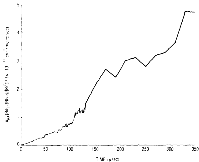
Fig. 9. Plot of Eq. (II) Constructed from the Absolute Data Presented in Fig. 8. The data from \text{BiF}(\text{AO}^+) used in this plot have had the scattered-light spike subtracted; an extrapolation from the remaining data was used for t < 30 \mu\text{sec} .
