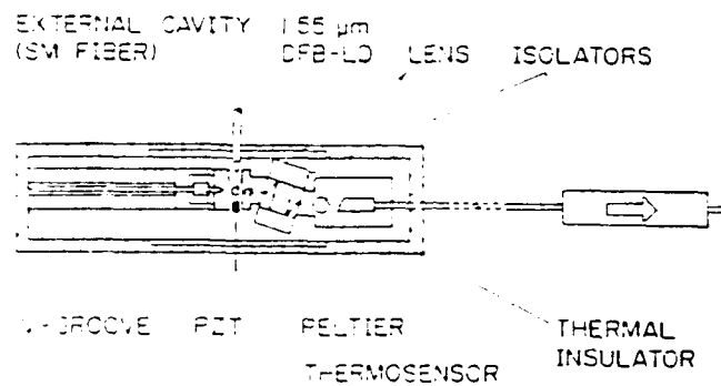
Fig. 6: Commerical DFB-ECSL module built by Fujitsu Labs. (Ref. 7) using single-mode fiber external cavity
