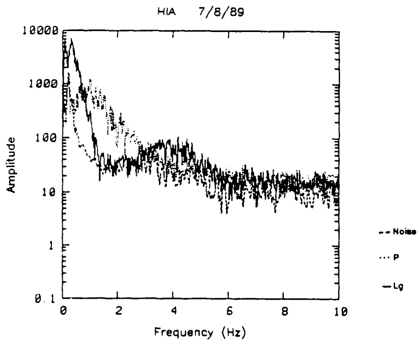
Figure 5. Regional P, L g and noise spectra measured at station HIA for Soviet nuclear tests at SR on 09/14/88 (JVE, top) and 07/08/89 (bottom).
