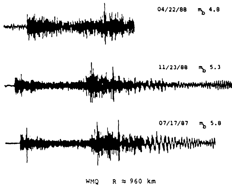
Figure 20. Examples of WMQ records from similar magnitude nuclear tests at SR and DM.
