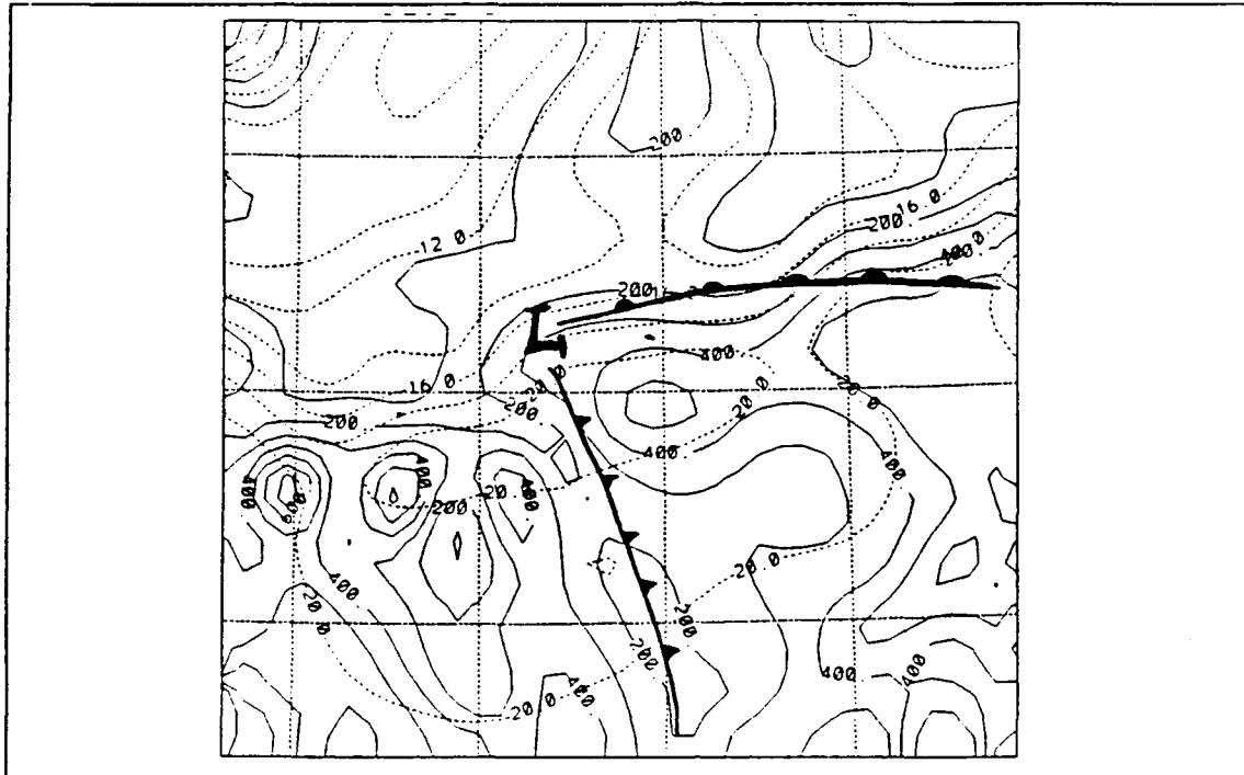
Figure 9. IOP-2 surface latent heat flux: Latent heat flux (solid) in W m^{-2} . SST (dashed) in ^{\circ}C . Grid as in Fig 7.
