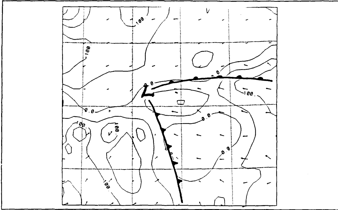
Figure 8. IOP-2 surface sensible heat flux: Sensible heat flux in W m^{-2} . Grid as in Fig. 7.
