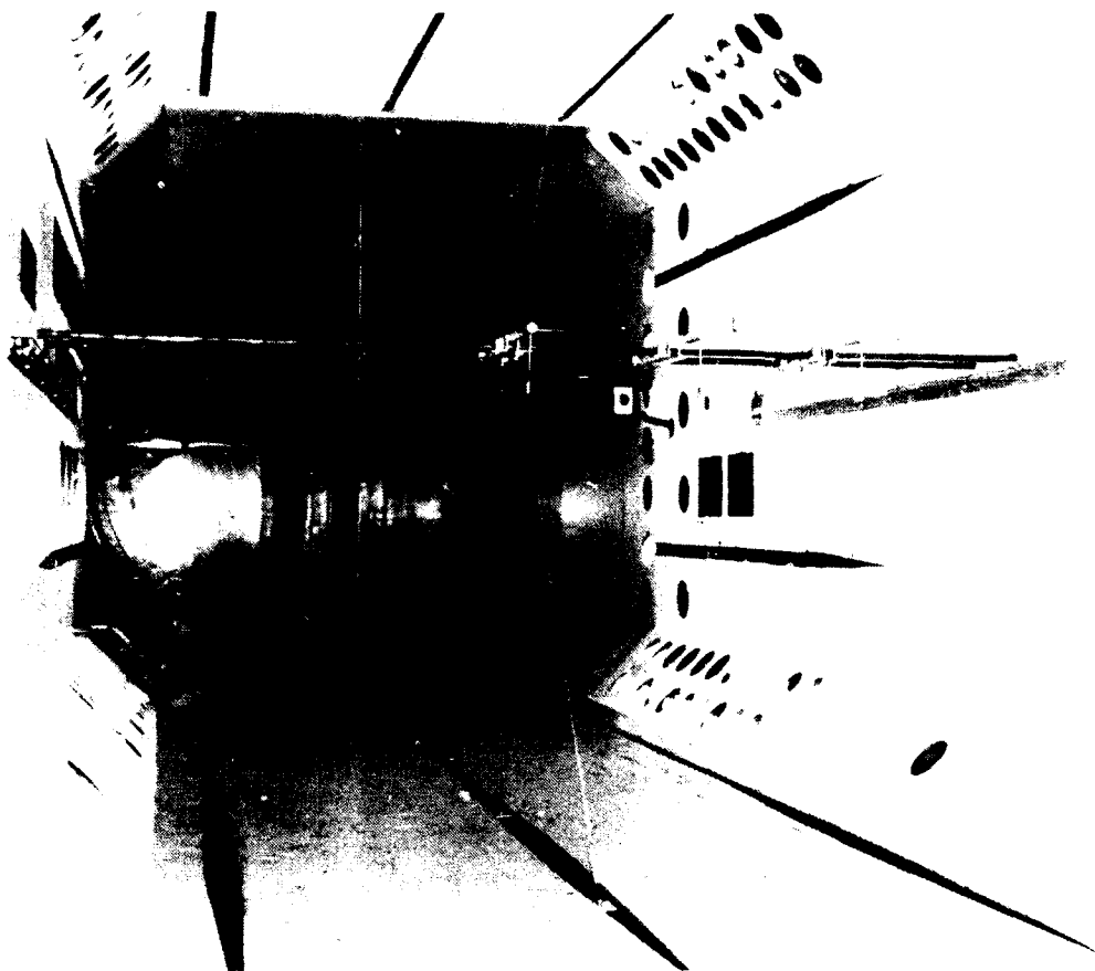
Figure 3. Airstream calibration rig mounted in Langley Transonic Dynamics Tunnel.
