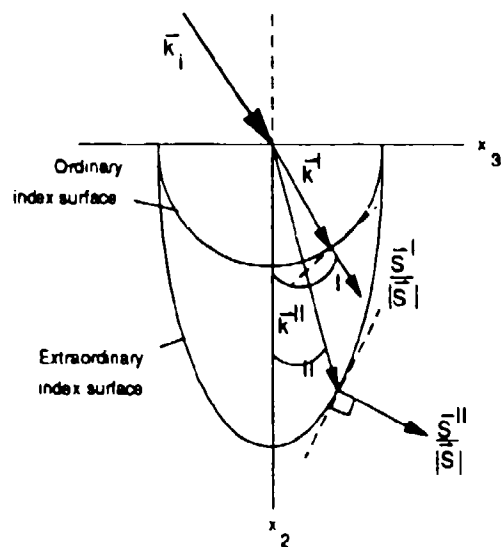
Figure 63. Propagation in a uniaxial crystal showing the effect of double-refraction at the interface and walkoff of the polarization in the plane of incidence (in the plane of the optic axis and the propagation vector).
