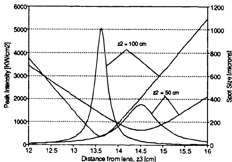
Figure 22. For a focal length of 12.5 cm, the plot shows the peak intensity and spot size as a function of the distance from the focussing element, z_3 , at the center of the ZnGeP_2 crystal for values of z_2 = 0.5 m (distance from the laser to the lens). These values have been normalized to an average power of 1 Watt at a pulse repetition frequency of 30 kHz.
