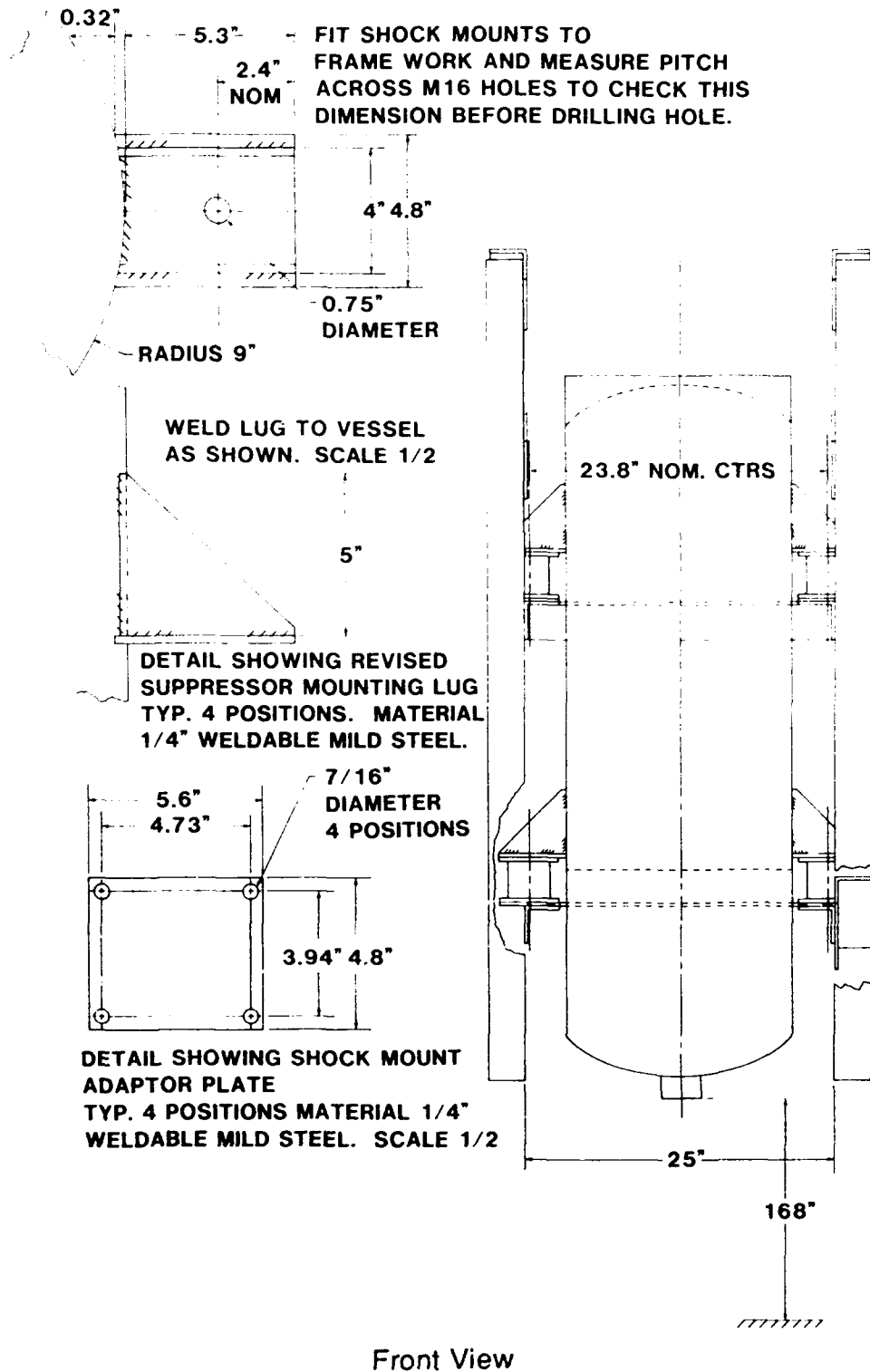
Figure 19. Company 'C' Cylinder Assembly with Shock Mount.
