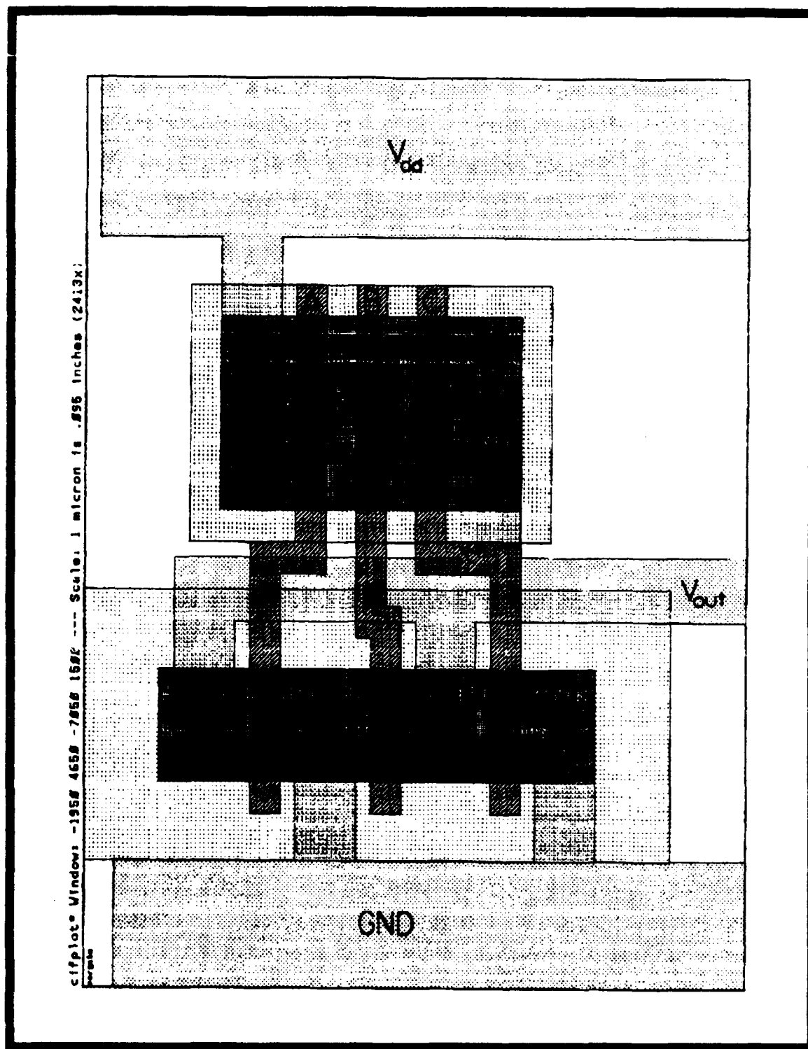
Figure E-5. 3-Input NOR gate layout.
