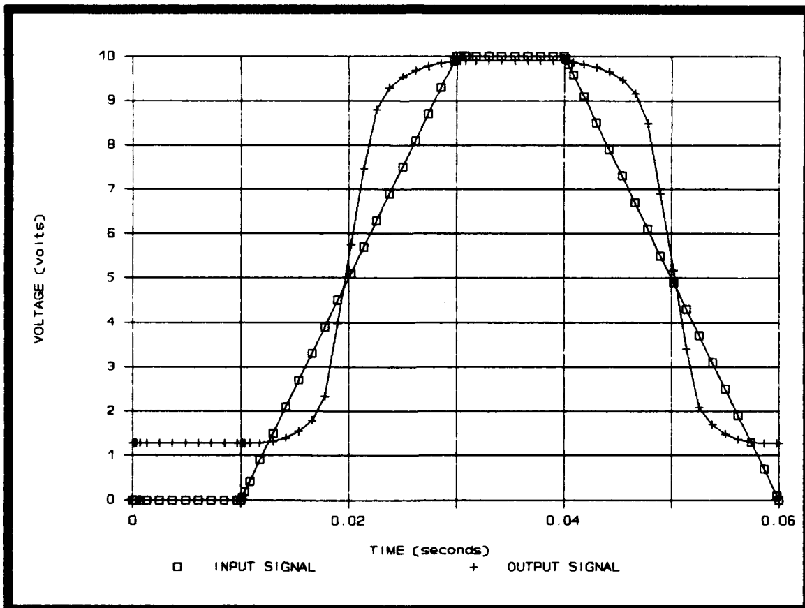
Figure D-1. Charge signal amplifier's output response to a piecewise-linear input.
