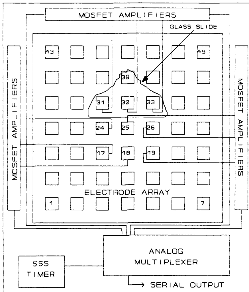
Figure 5-17. Location of the glass slide for the shape recognition test.
